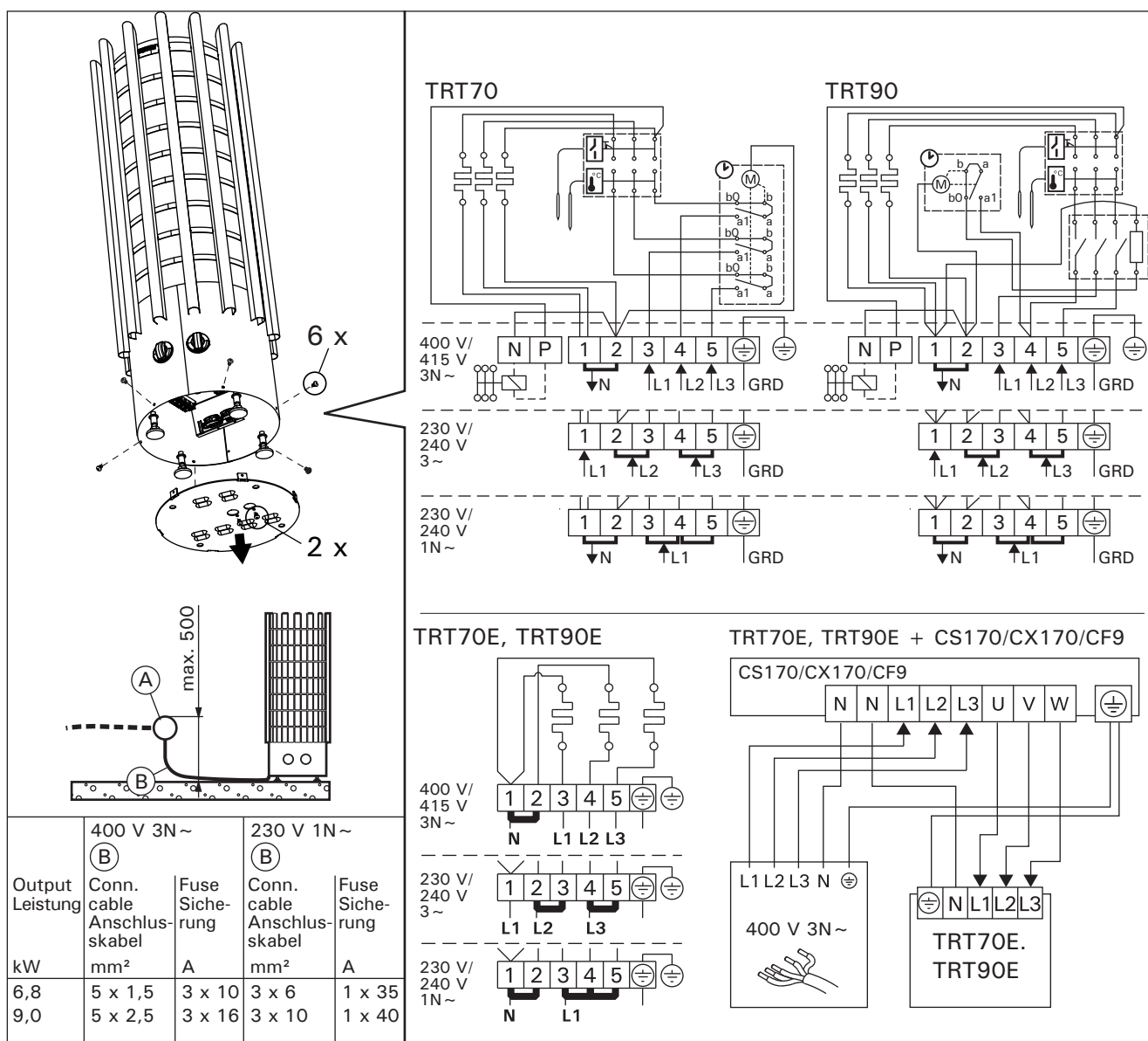
Figure 7. Electrical connections Abbildung 7. Elektroanschlüsse
