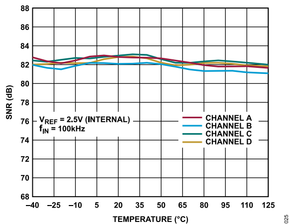
Figure 25. SNR vs. Temperature
