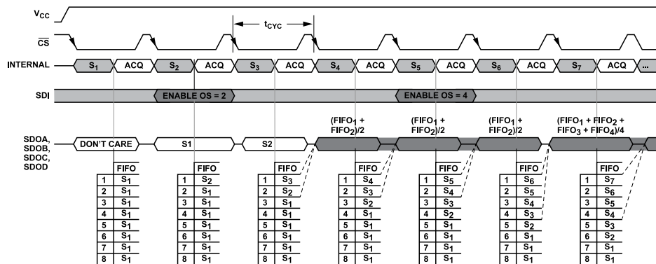
Figure 40. Rolling Average OS Mode Configuration
