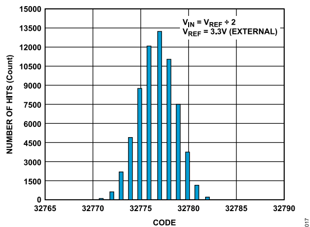
Figure 17. DC Histogram
