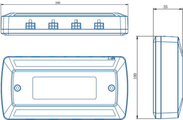
JCB35H7B1dimension and connection
