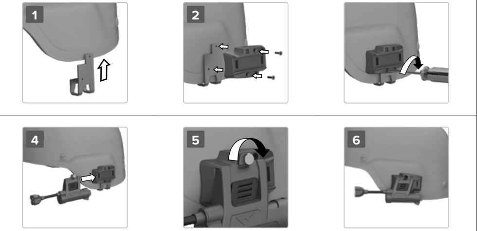
Figure 8 – Picatinny Rail Mount
