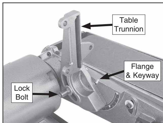
Figure 13. Sanding belt table trunnion installed.
