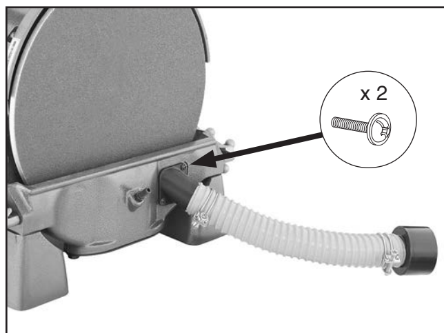
Figure 17. Sanding disc dust hose assembly attached.
