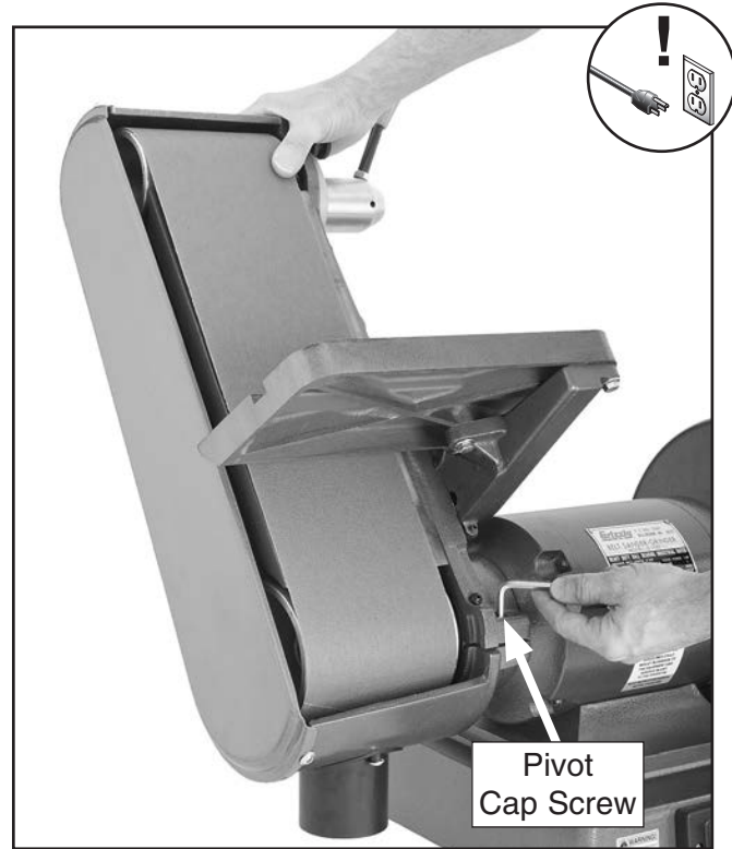
Figure 36. Positioning the sanding belt assembly.
