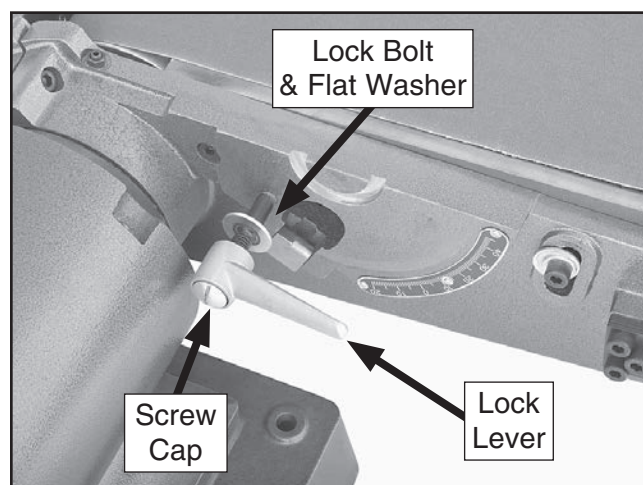
Figure 12. Sanding belt lock lever.
