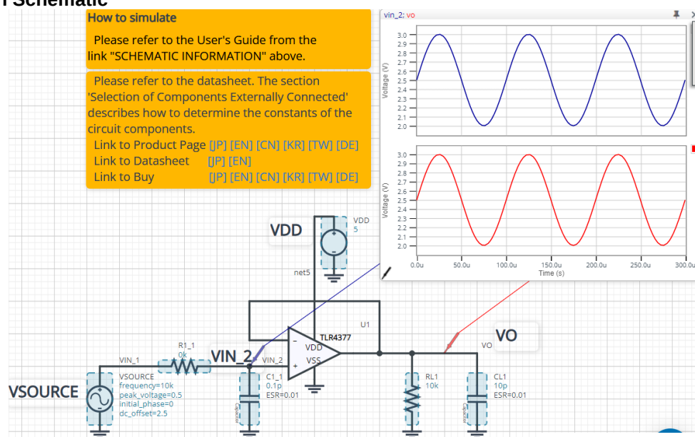
Figure 1. Simulation Schematic
