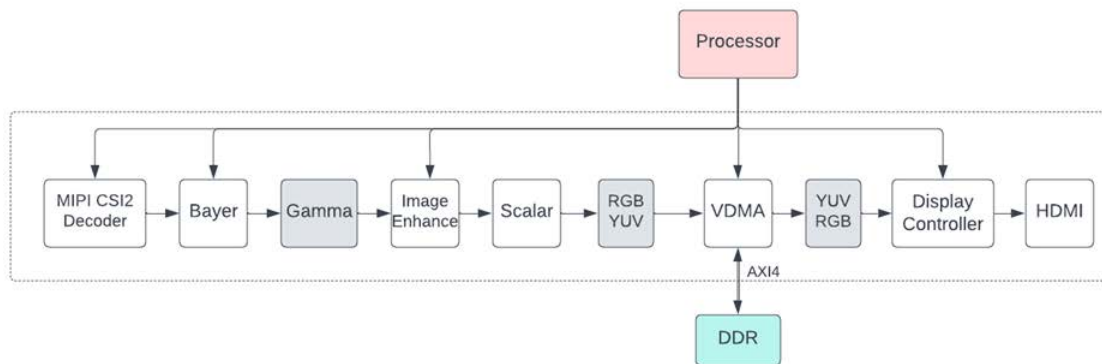
Figure 6-16. Video Pipeline Architecture
