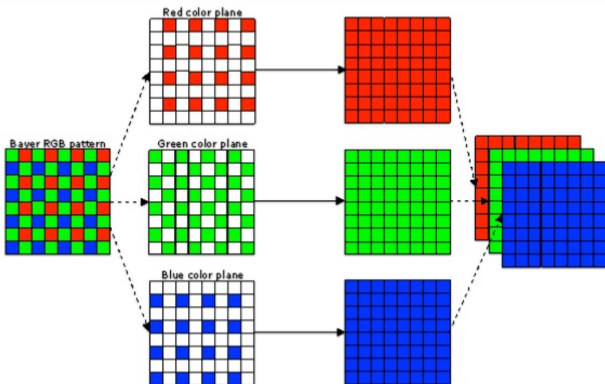
Figure 6-18. Demosaicing of Bayer Format Image
