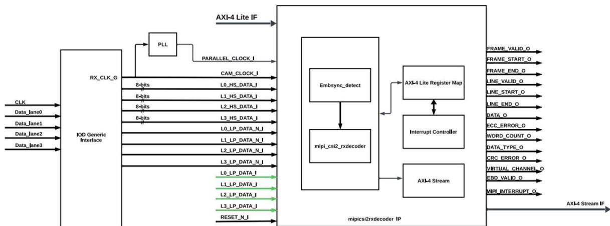
Figure 6-19. Block Diagram MIPI CSI-2 Input
