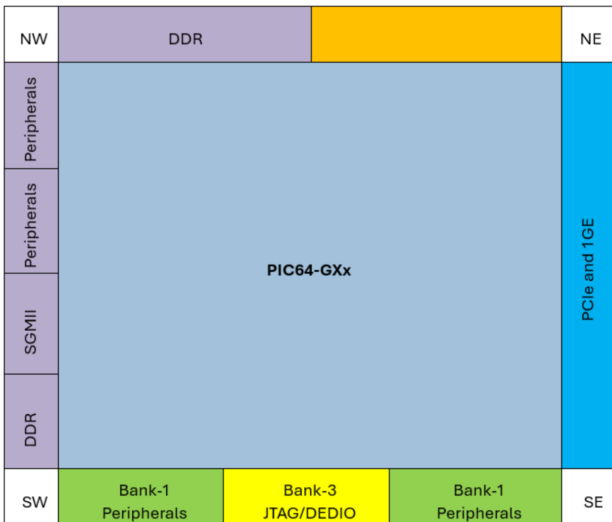
Figure 14-2. Package/IO Locations
