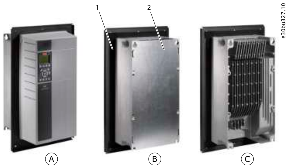
Figure 13: Panel Through Mounting Kit on a VLT® Drive
