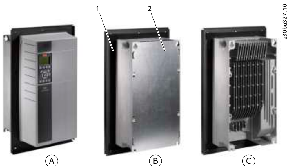
Figure 12: Panel Through Mounting Kit on a VLT® Drive
