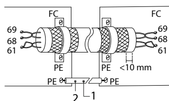
Figure 68: Twisted-pair Cables
