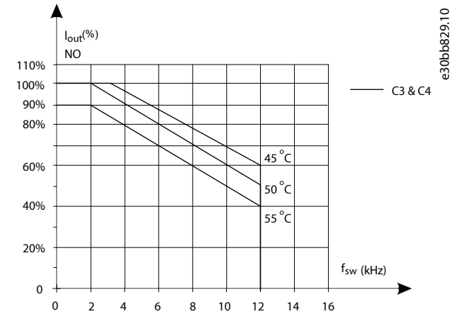
Figure 52: Derating of I_{out} for Different T_{AMB,MAX} for Enclosure Sizes C3 and C4, using 60° AVM
