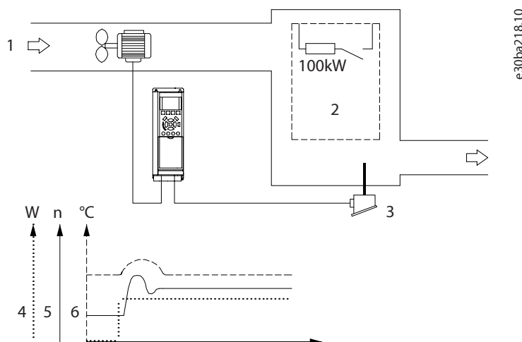
Figure 101: Closed-loop Control in a Ventilation System
