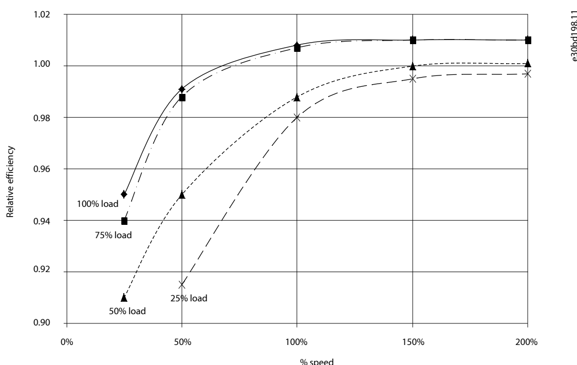
Figure 85: Typical Efficiency Curves
