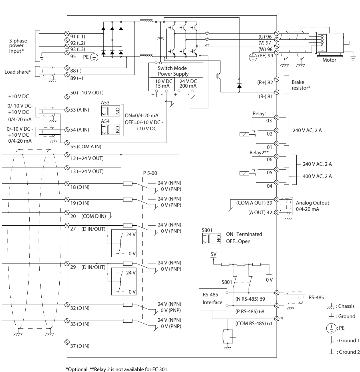
Figure 64: Basic Wiring Schematic
