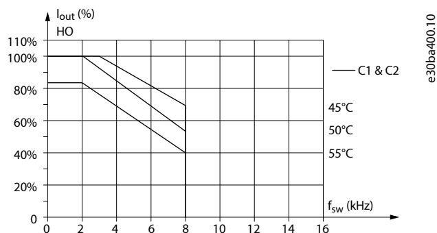
Figure 53: Derating of I_{out} for Different T_{amb,MAX} for Enclosure Sizes C1 and C2, using SFAVM
