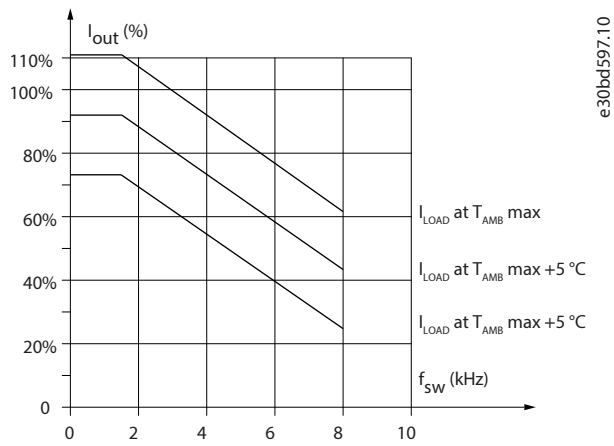
Figure 63: Output Current Derating with Switching Frequency and Ambient Temperature for Enclosure Size C3
