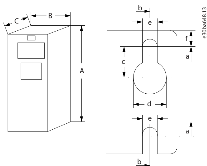
Figure 25: Top and Bottom Mounting Holes
