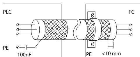
Figure 67: Connection with a 100 nF Capacitor
