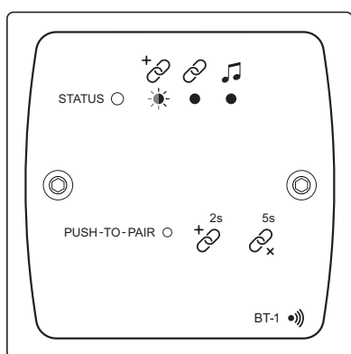
BT-1 Bluetooth wireless audio input module
