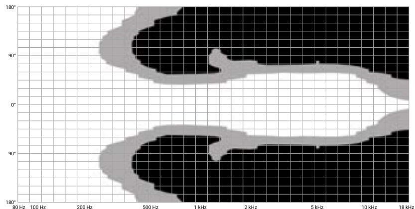
CS7 Horizontal Pattern
