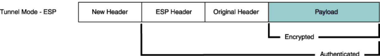
Figure 19: Tunnel Mode
