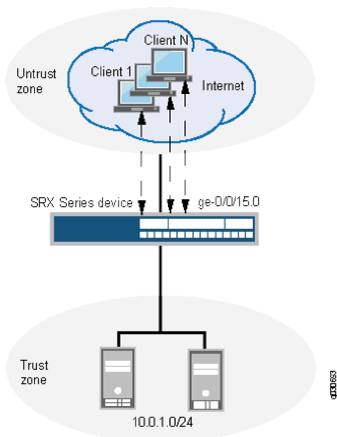
Figure 73: Dynamic VPN Deployment Topology
