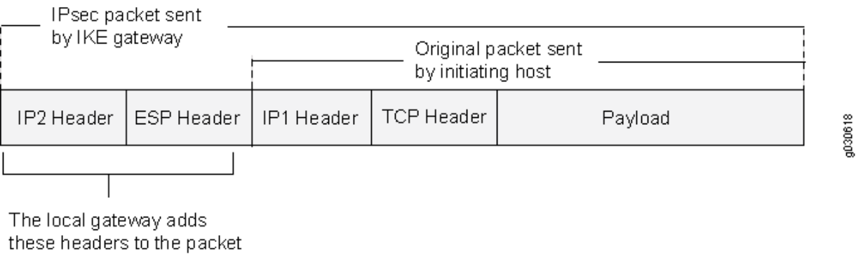
Figure 13: IPsec Packet—ESP in Tunnel Mode
