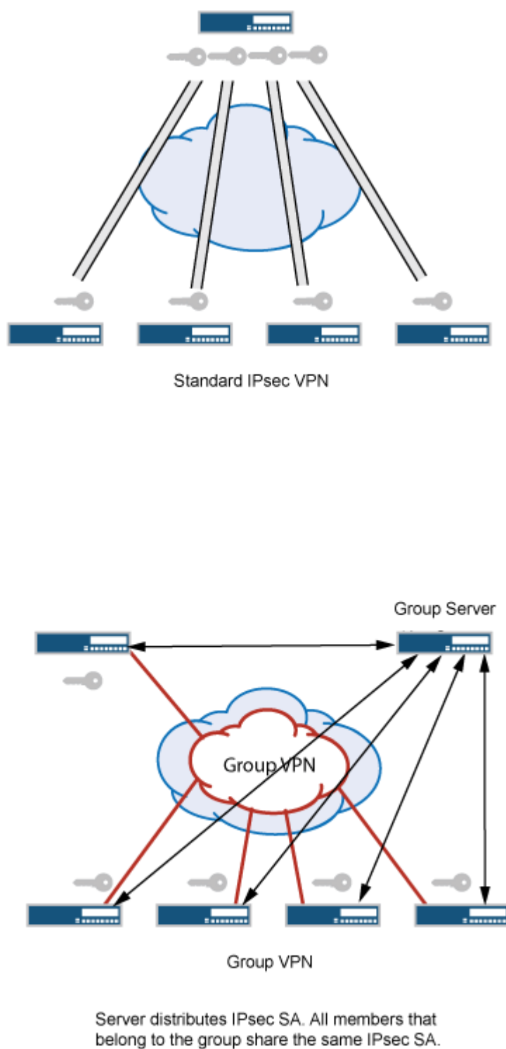
Figure 46: Standard IPsec VPN and Group VPNv1
