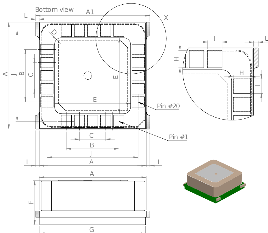
Figure 3 Dimensions
