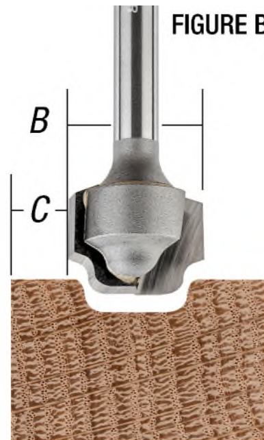
A: Base Diameter B: Bit Diameter C: Desired Offset from Edge
