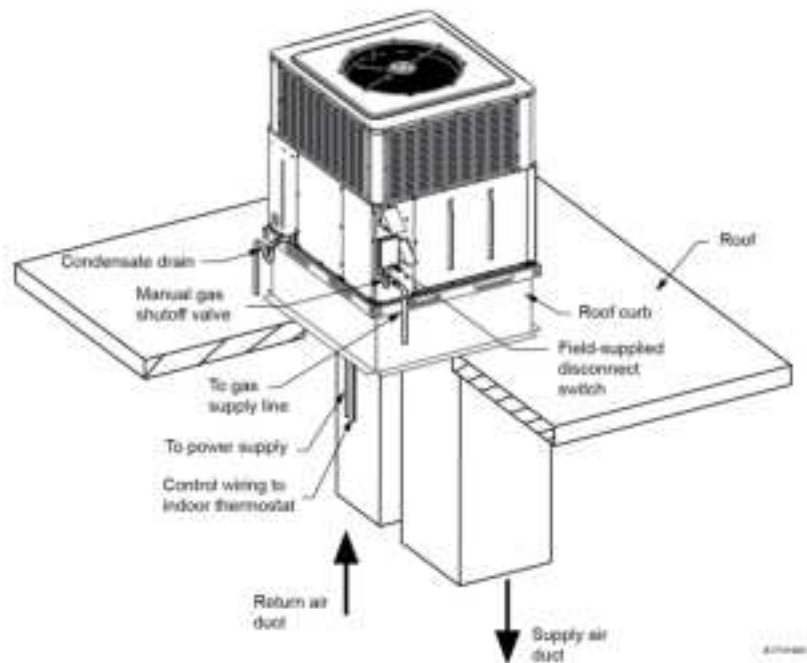
Figure 8: Typical installation on roof curb for unit
