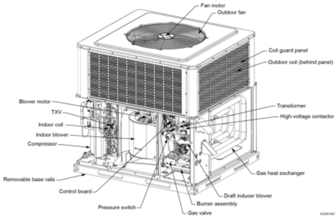
Figure 1: Unit components - PG3E36, PG3E48, and PG3E60 units
