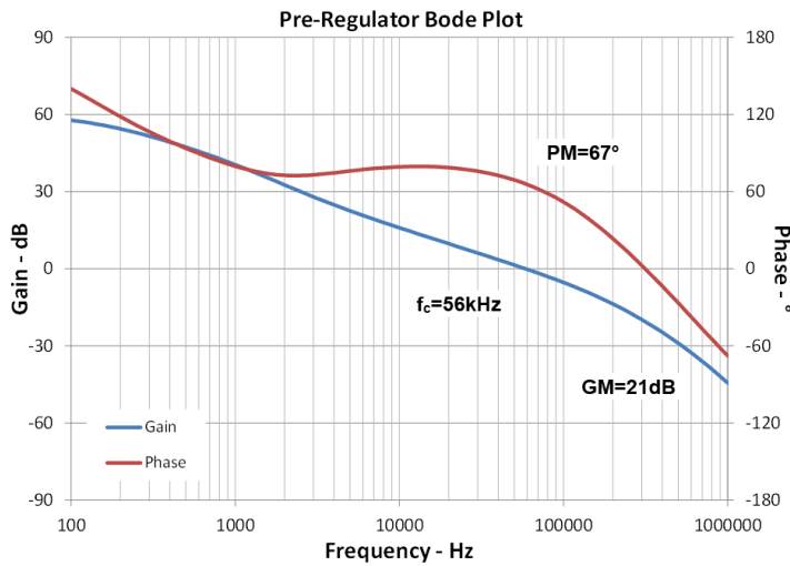
Figure 9: Bode Plot for Pre-Regulator
