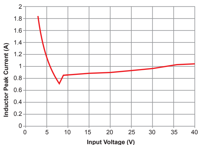
Figure 8: Typical Peak Inductor Current versus Input Voltage for 0.8 A Output Current and 10 \mu\text{H} Inductor
