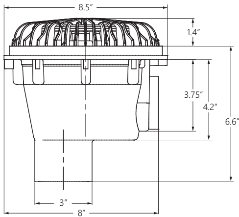
NOVA - SIDE VIEW
