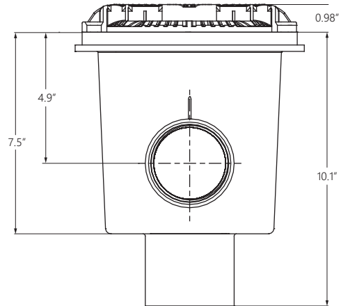
LARGE OUTLET NOVA - SIDE VIEW A
