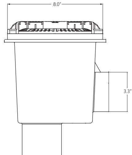
LARGE OUTLET NOVA - SIDE VIEW B
