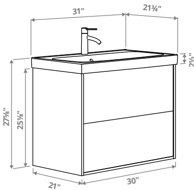
HAVBÄCK/ORRSJÖN Sink cabinet with drawers/sink/faucet, 31×21¾×27⅝".
