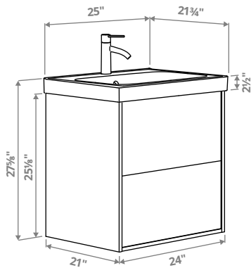
HAVBÄCK/ORRSJÖN Sink cabinet with drawers/sink/faucet, 25×21¾×27⅝".
