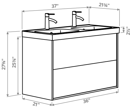
HAVBÄCK/ORRSJÖN Sink cabinet with drawers/sink/faucets, 37⅛×21¾×27⅝".
