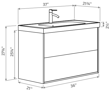
HAVBÄCK/ORRSJÖN Sink cabinet with drawers/sink/faucet, 37⅛×21¾×27⅝".
