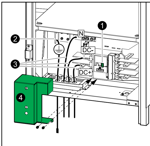
Empty Battery Cabinet – Bottom Cable Entry
