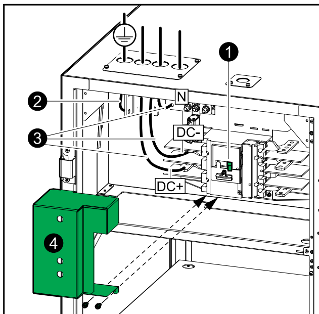
Empty Battery Cabinet – Top Cable Entry
