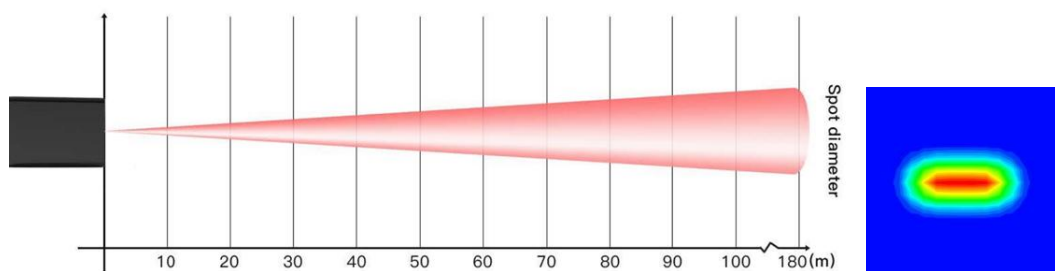
Figure. 3: FoV of TFA170-L
