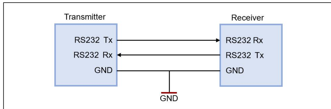
Figure. 6: RS-232 Connection Diagram
