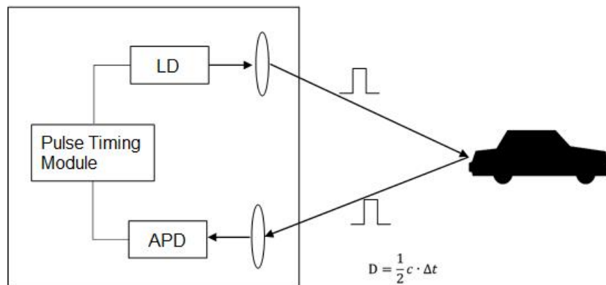
Figure. 1: Pulsed time of flight
