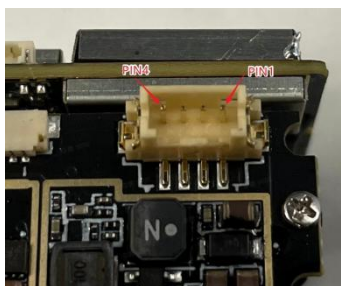
Figure. 5: LiDAR connector appearance
