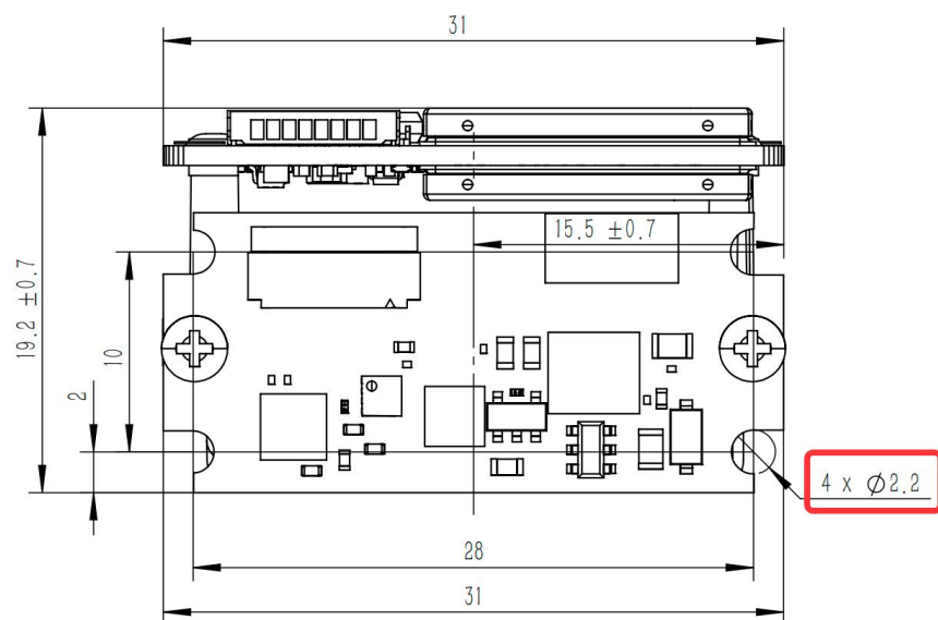
Figure. 4: Diagram of TFA170-L installation hole
