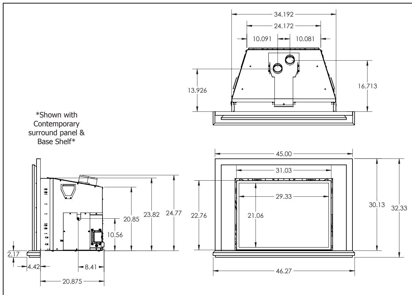
Figure 1: E44I Exterior Dimensions.
