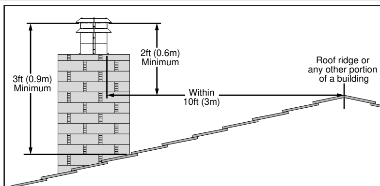
Figure 26: Roof Clearances.
