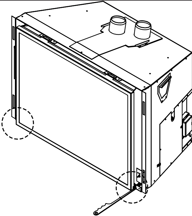
Figure 19: Door Release.
