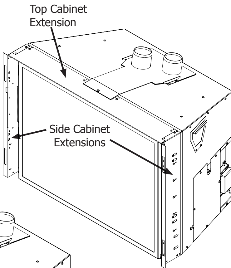
Figure 44: Stove as Shipped
