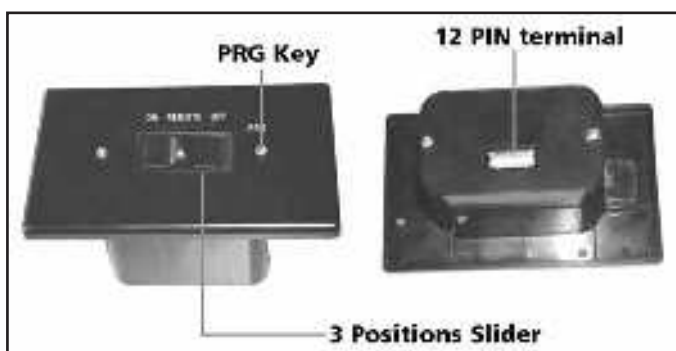
Figure 8: Proflame Receiver.
