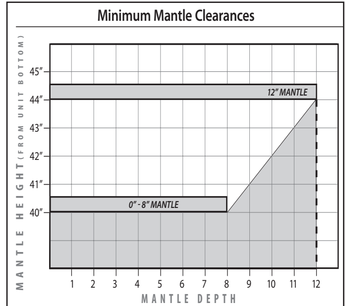
Figure 25: Mantle width and height.
