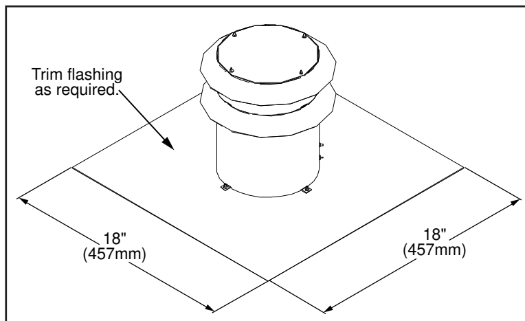
Figure 29: Generic Vent Cap Dimensions.
