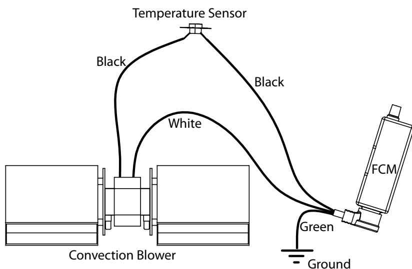
Figure 23: Fan Wiring.
