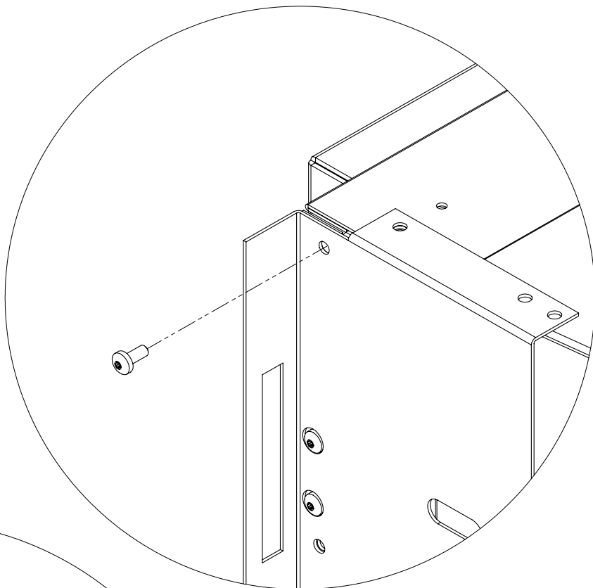
Figure 42: Top Extension Screw Removal
