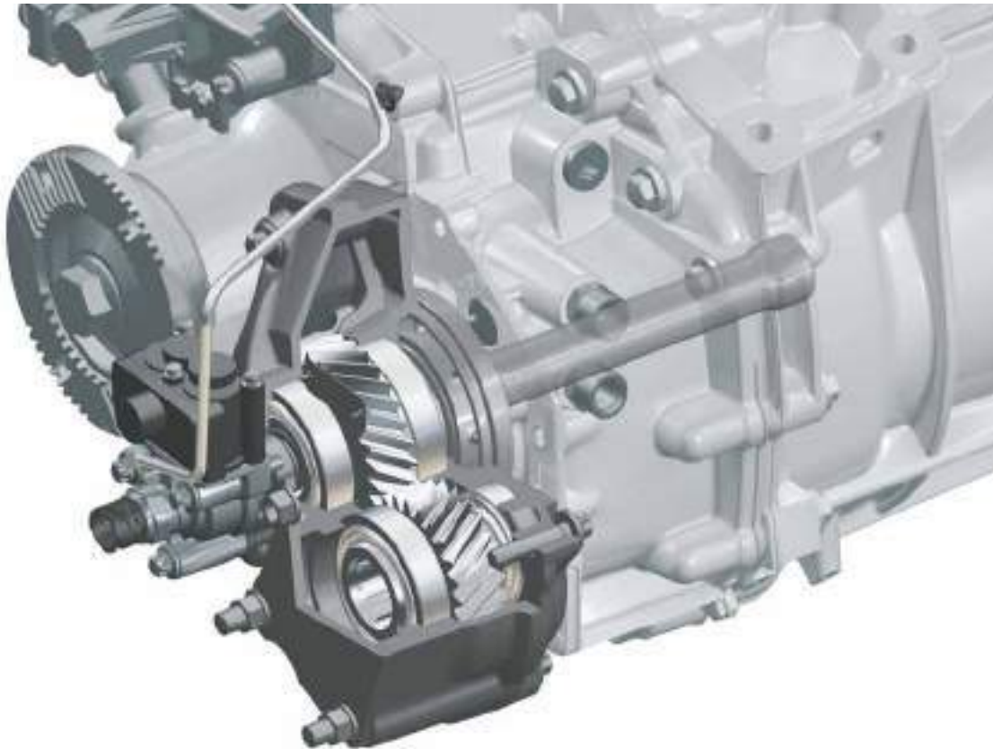
Power take-off NA MB 131-2c, pump (N2E) on transmission G 141-9
