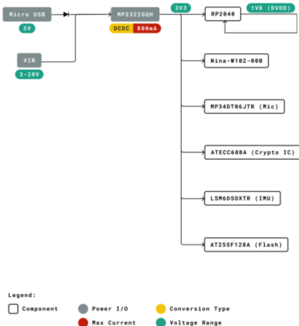
Power Tree of Arduino Nano RP2040 Connect Topology
