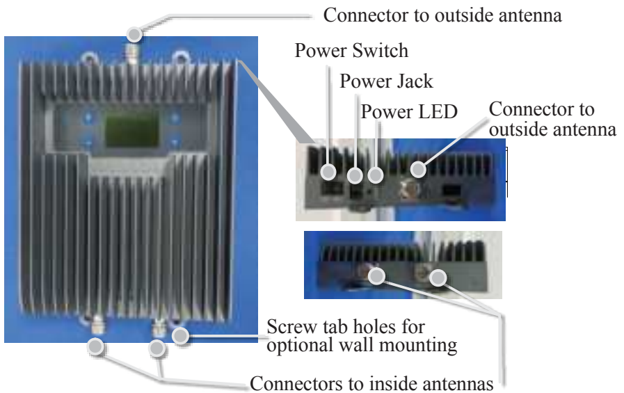
Host Unit Diagram
