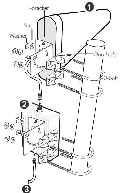
Outside system assembly
