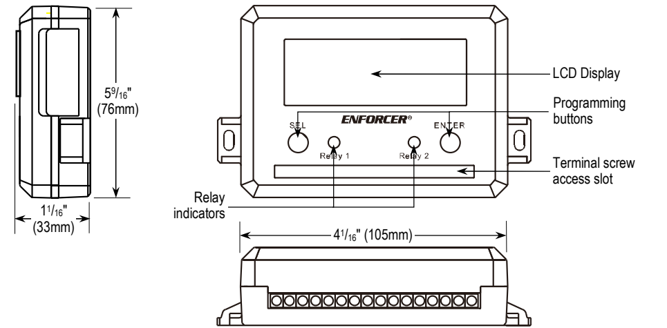
Terminal Layout Chart (left to right)
