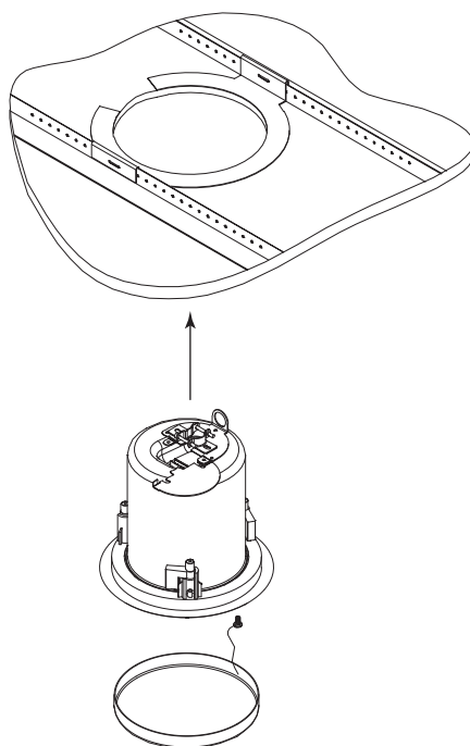
Figure 16: Mount speaker into ceiling
