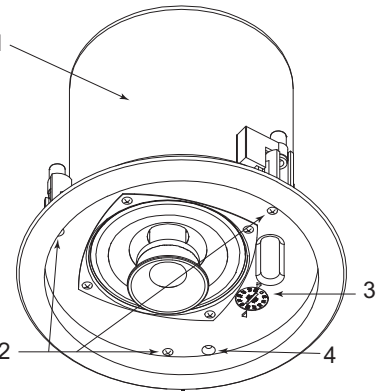
Figure 2: Bottom of speaker
