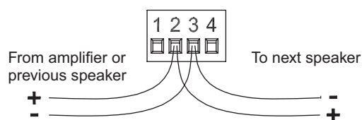
Figure 9: Parallel wiring
