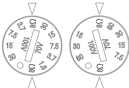
Figure 19: Adjust tap selector (left: C4.2/C8.2/C8.2LP; right: C10.1/C8.2HC)
