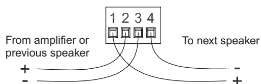
Figure 10: Daisy-chain wiring
