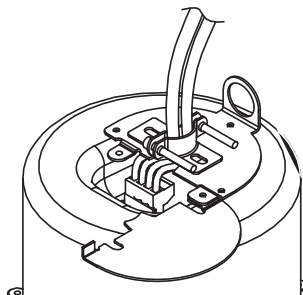
Figure 14: Secure cable through fitting
