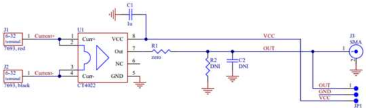
Figure 3: CT4022 Evaluation Board Schematic
