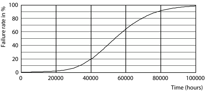
Life Expectancy Diagram - MAS LEDtube VLE 1200mm HO 16W 865 T8 SL
