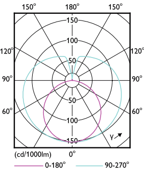
Light Distribution Diagram - MAS LEDtube VLE 1200mm HO 16W 865 T8 SL
