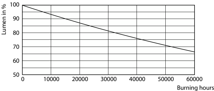
Lumen Maintenance Diagram - MAS LEDtube VLE 1200mm HO 16W 865 T8 SL
