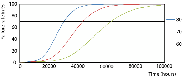
Life Expectancy Diagram - MAS LEDtube VLE 1200mm HO 16W 865 T8 SL
