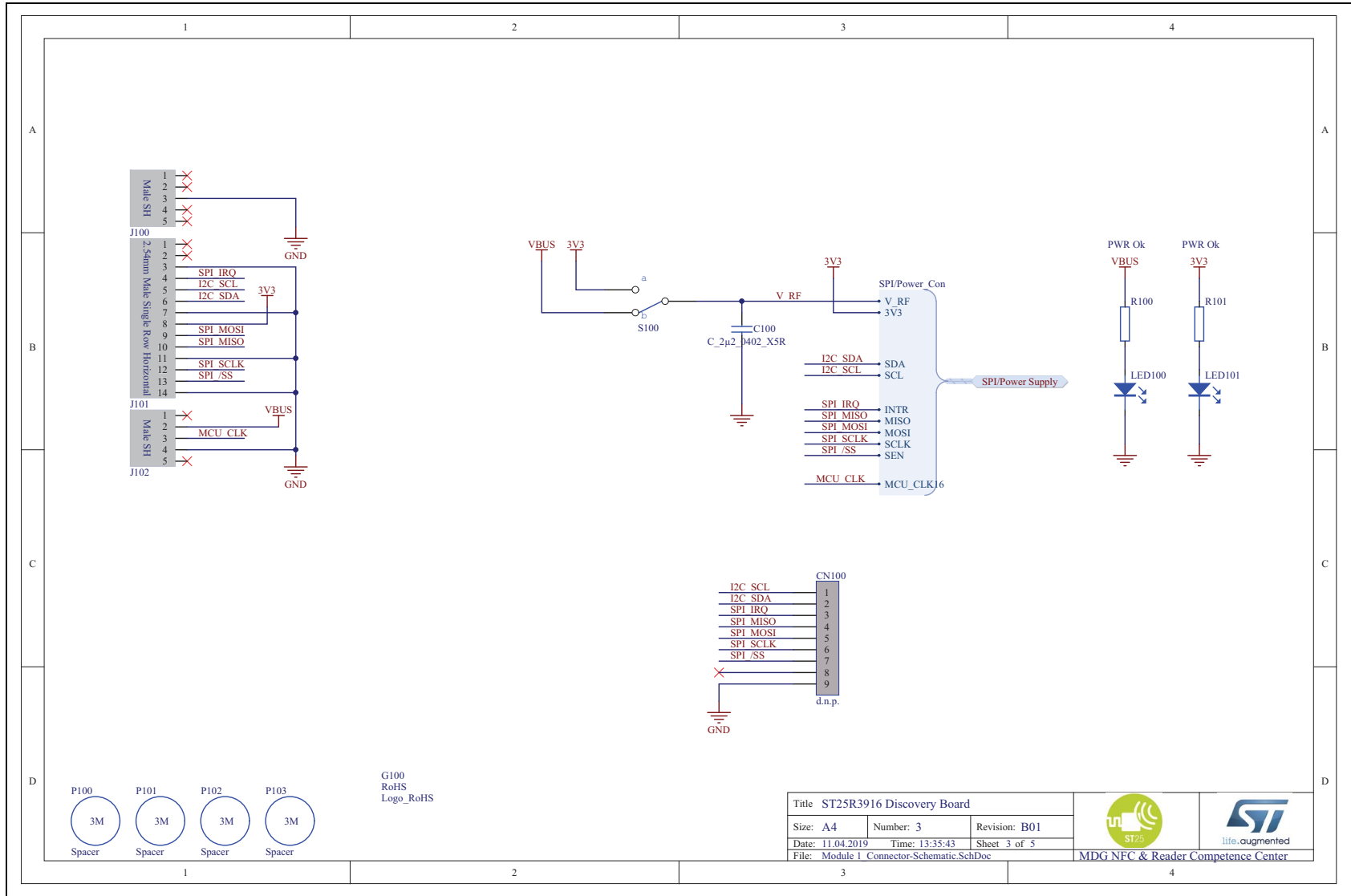
Figure 19. MB1414 - Connectors
