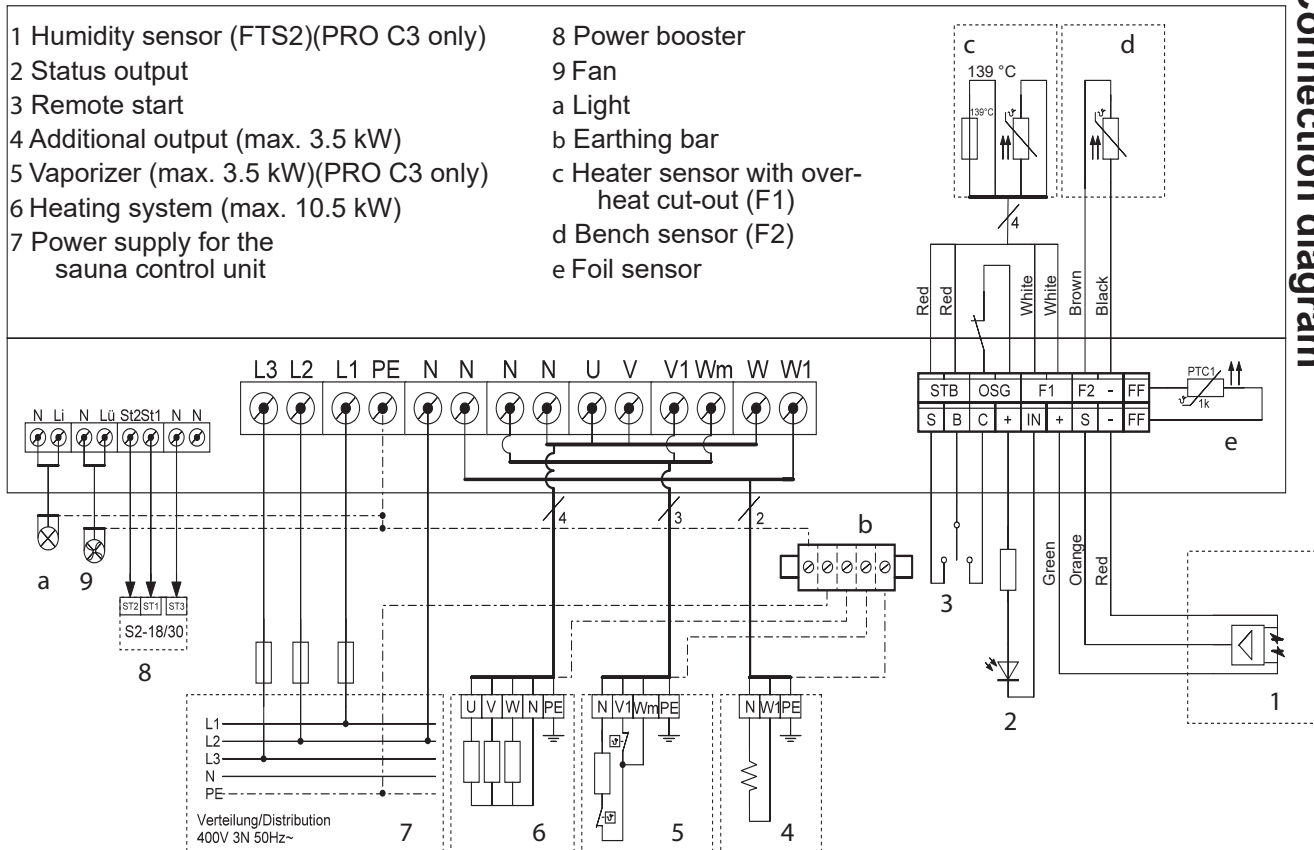
Fig.4 Connection diagram
