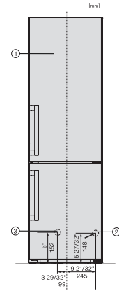
KFN4799DDE, installation (footnote*) (installation drawings) (US)
