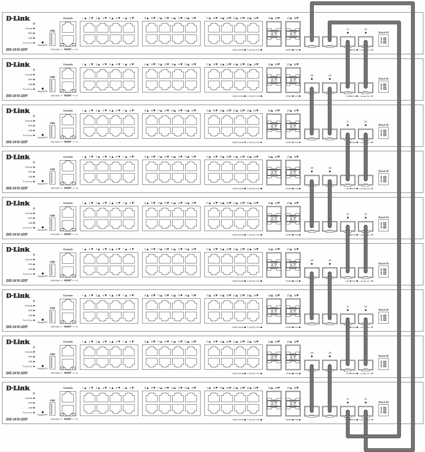
Figure 4-2 Duplex Ring Stacking Topology
