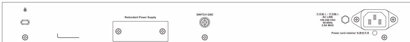
Figure 2-6 DXS-3410-32SY Rear Panel
