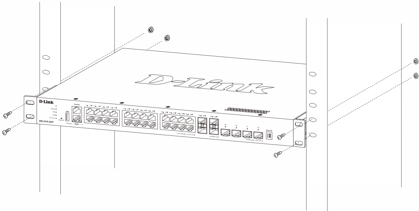
Figure 3-3 Installing the Switch in a Rack
