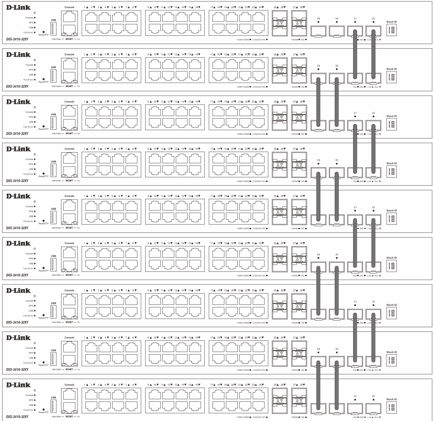
Figure 4-1 Duplex Chain Stacking Topology
