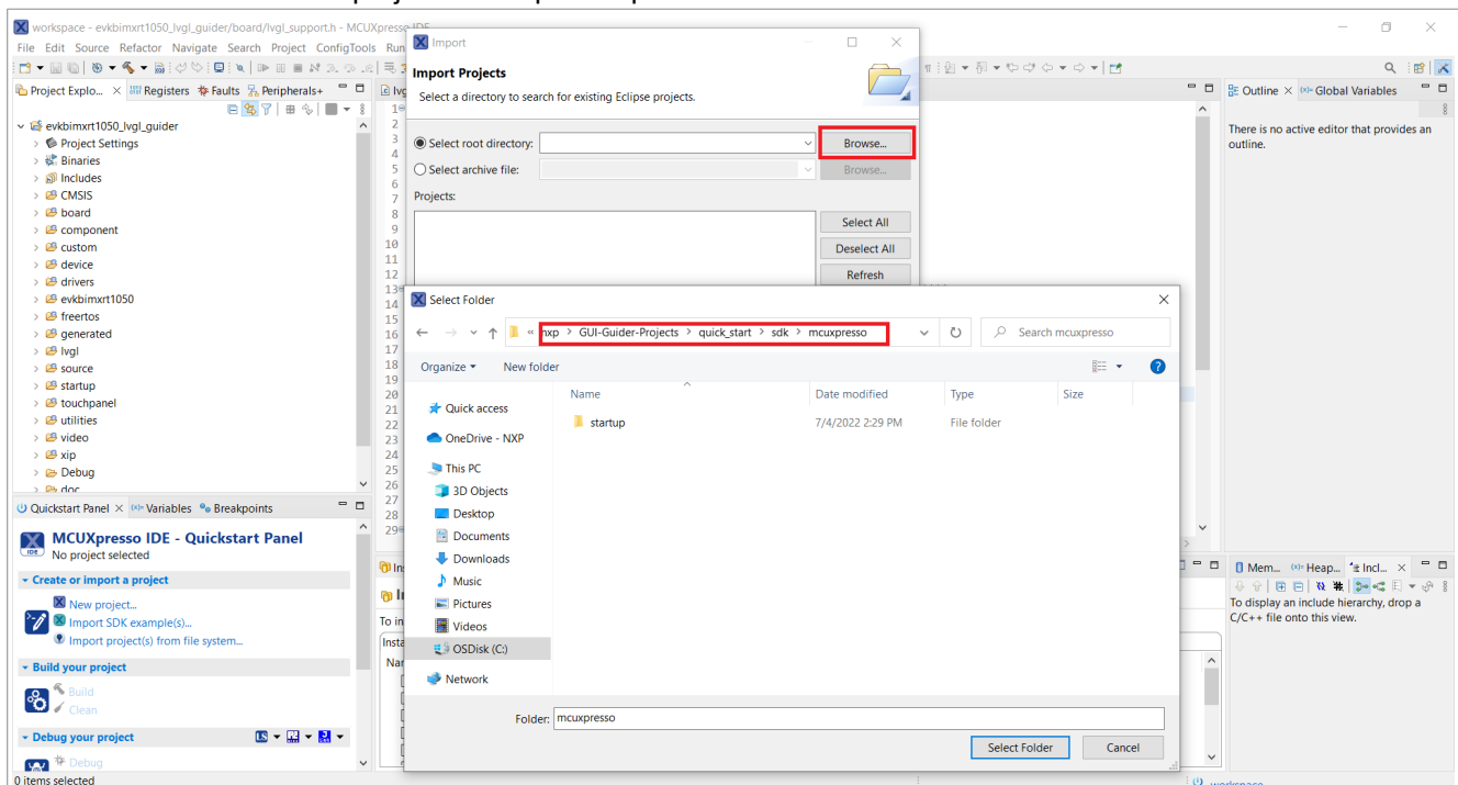
Figure 143. Selecting the GUI Guider project path
