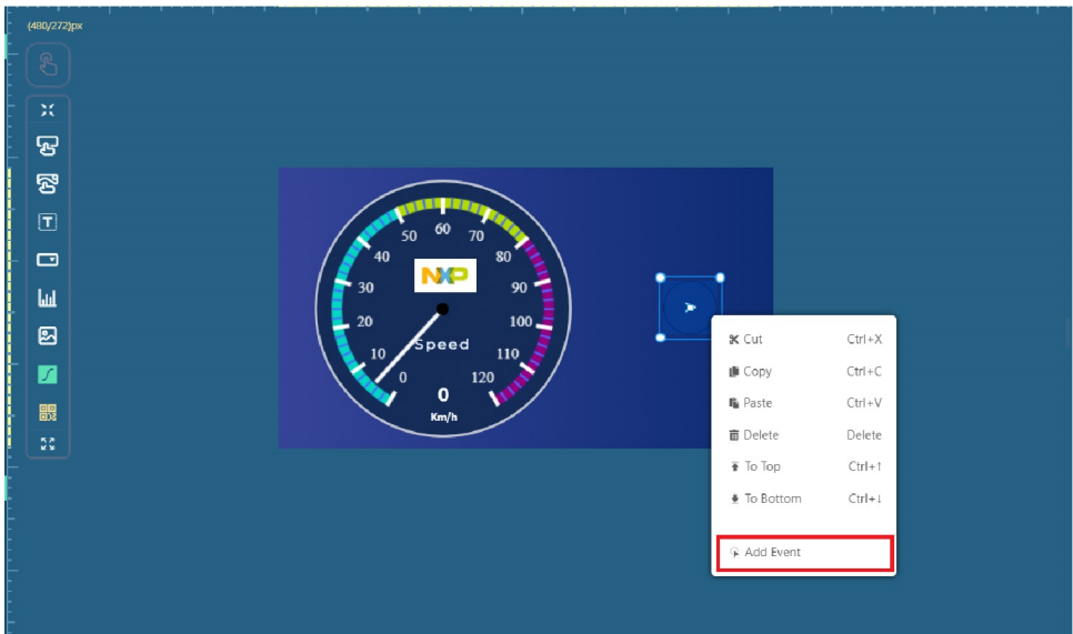
Figure 36. Add event
