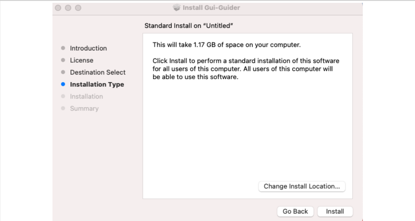
Figure 5. Click 'Install'
