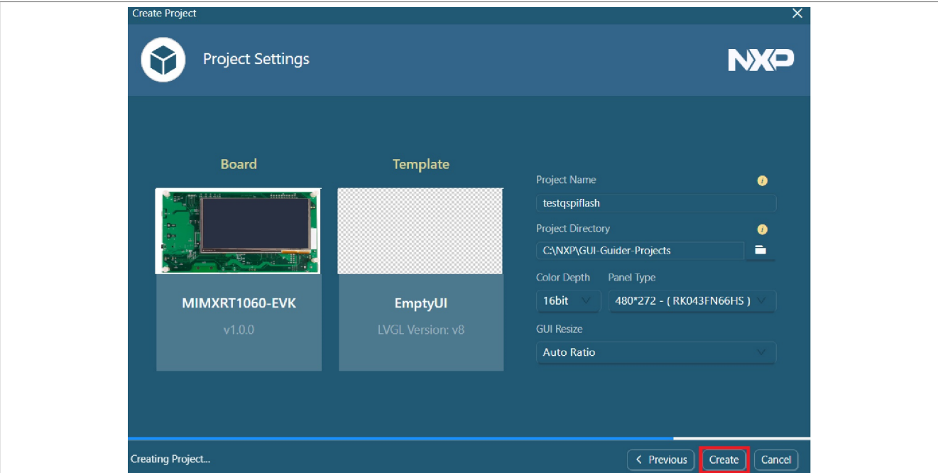
Figure 176. Project settings
