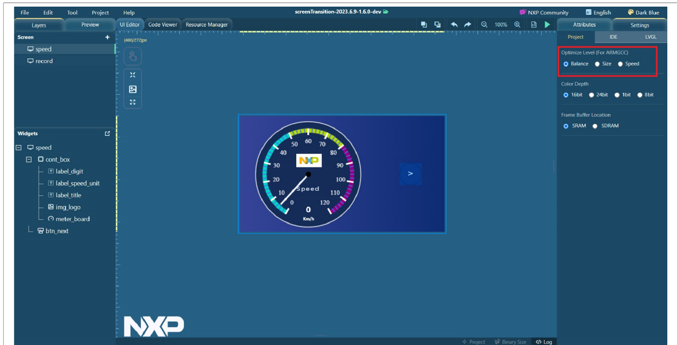
Figure 139. Optimization level
