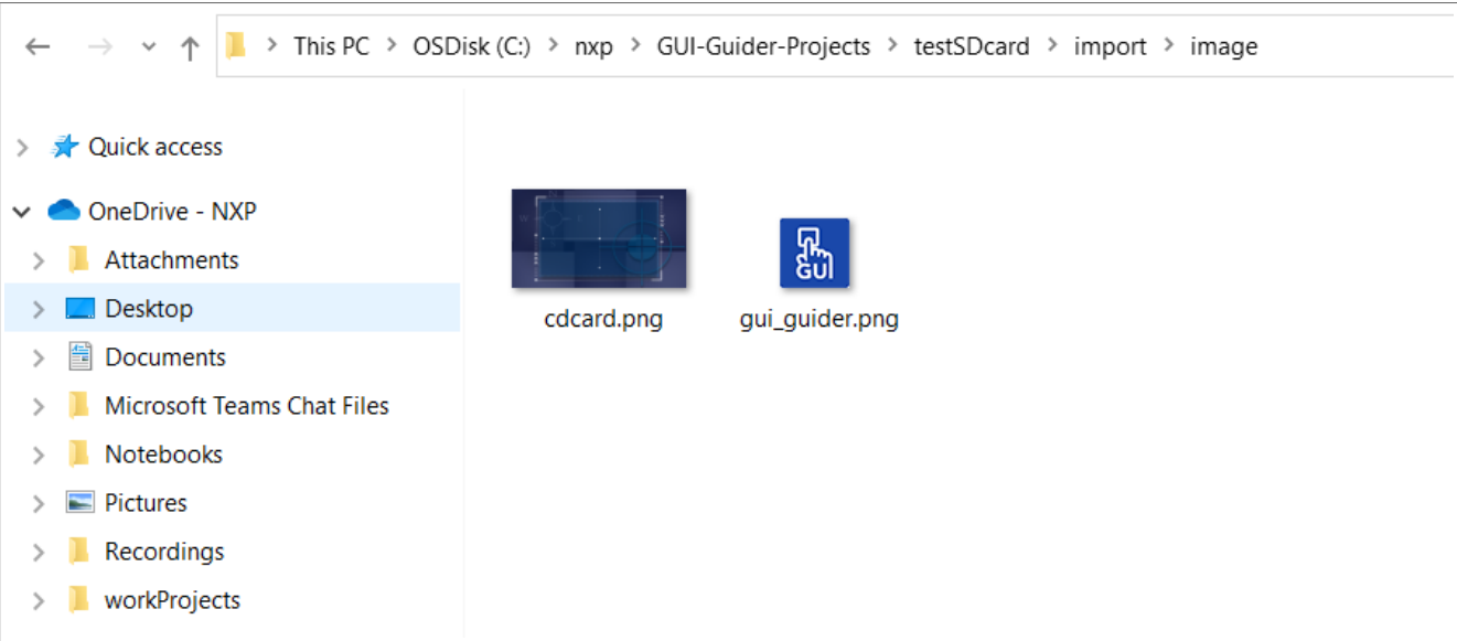
Figure 170. Import folder
