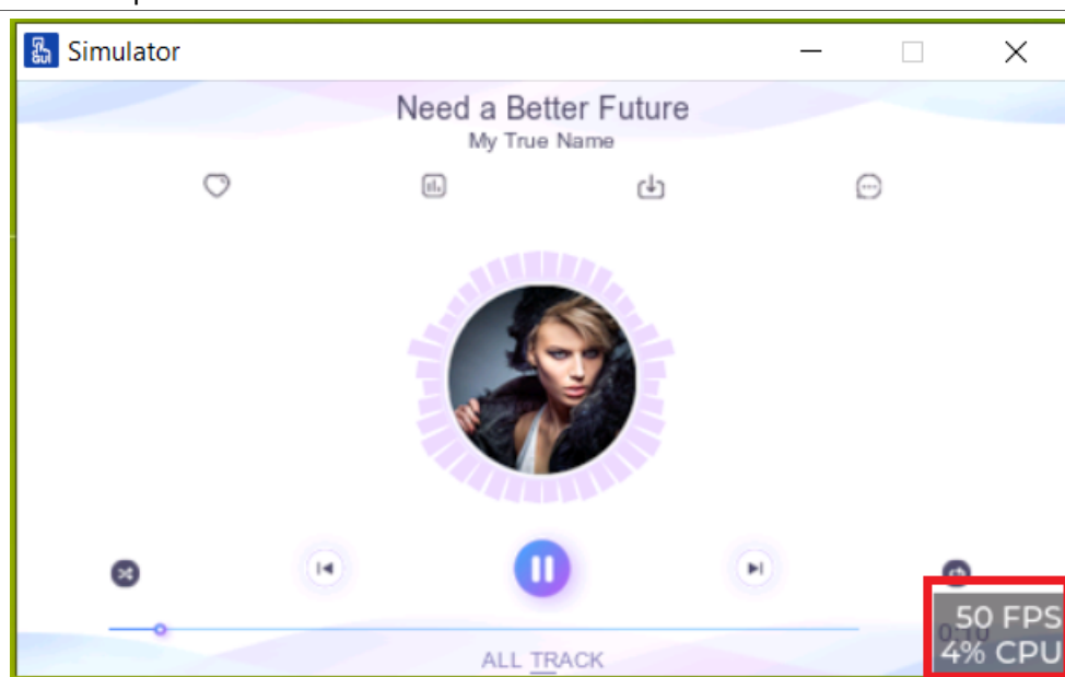
Figure 137. Performance monitor
