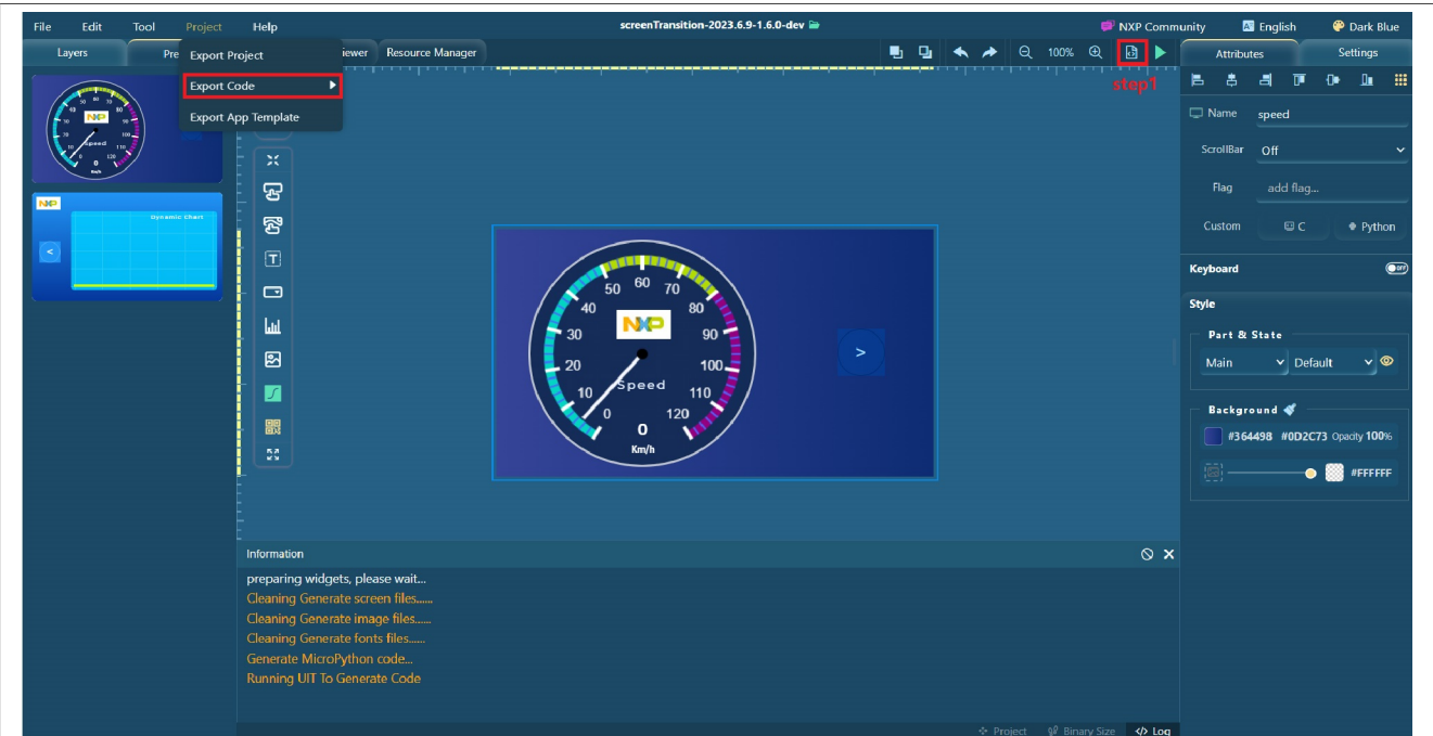
Figure 23. Exporting code
