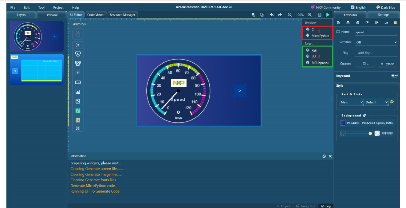
Figure 29. Running simulator
