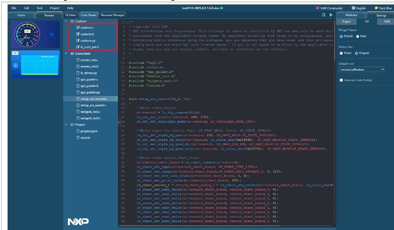
Figure 28. Code view
