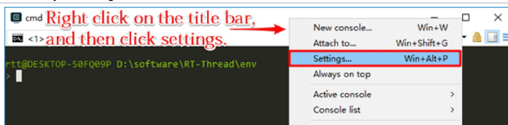
Figure 149. Click settings
