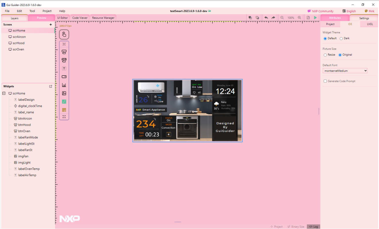
Figure 47. Pink theme
