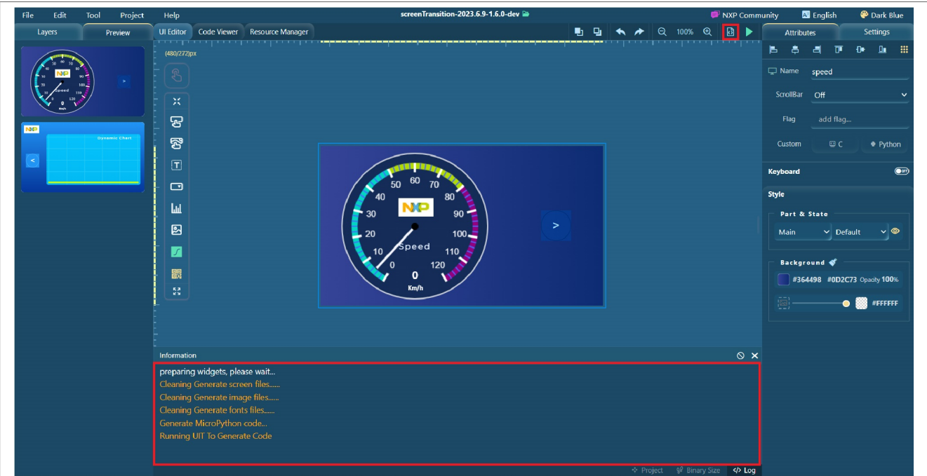
Figure 22. Generating code
