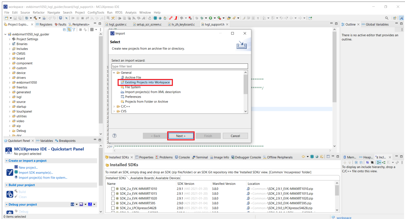
Figure 142. Importing project
