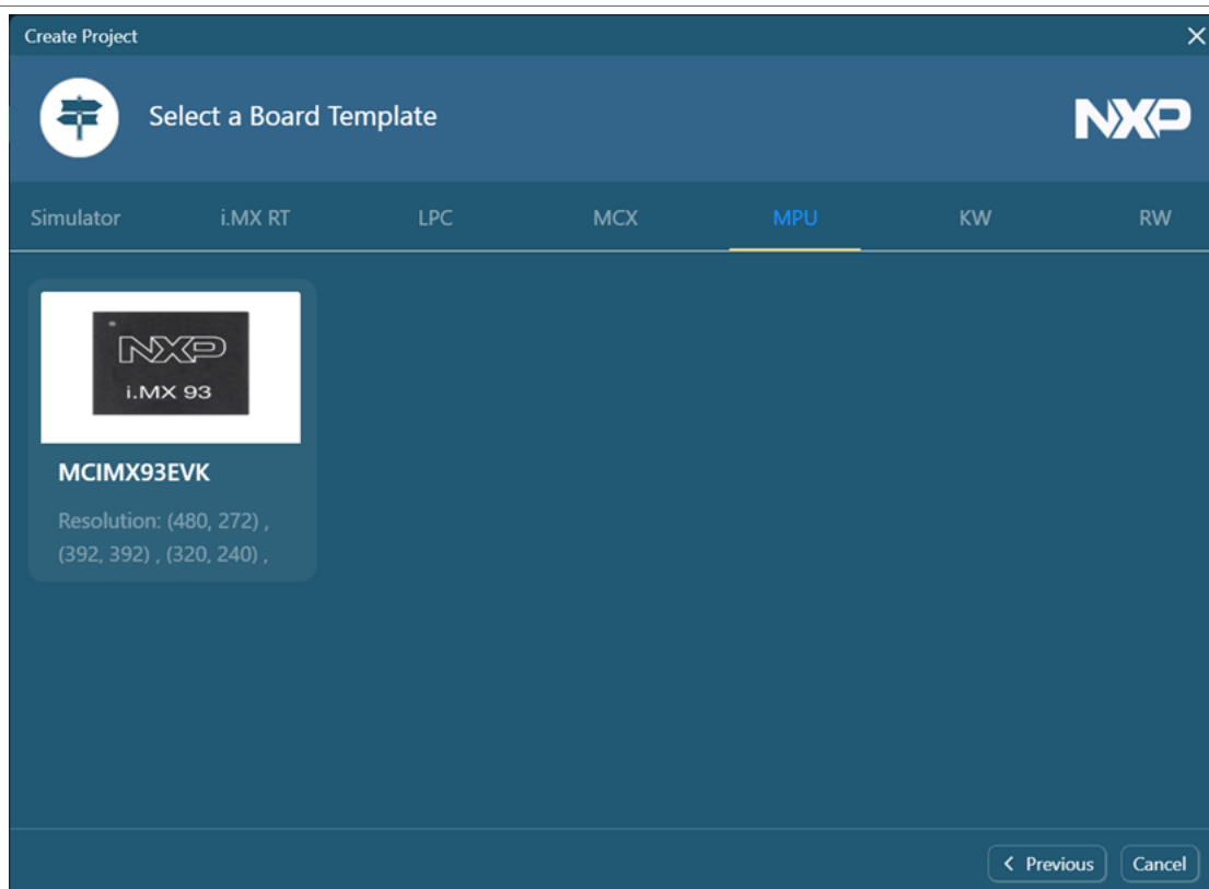
Figure 161. Select MCIMX93EVK template
