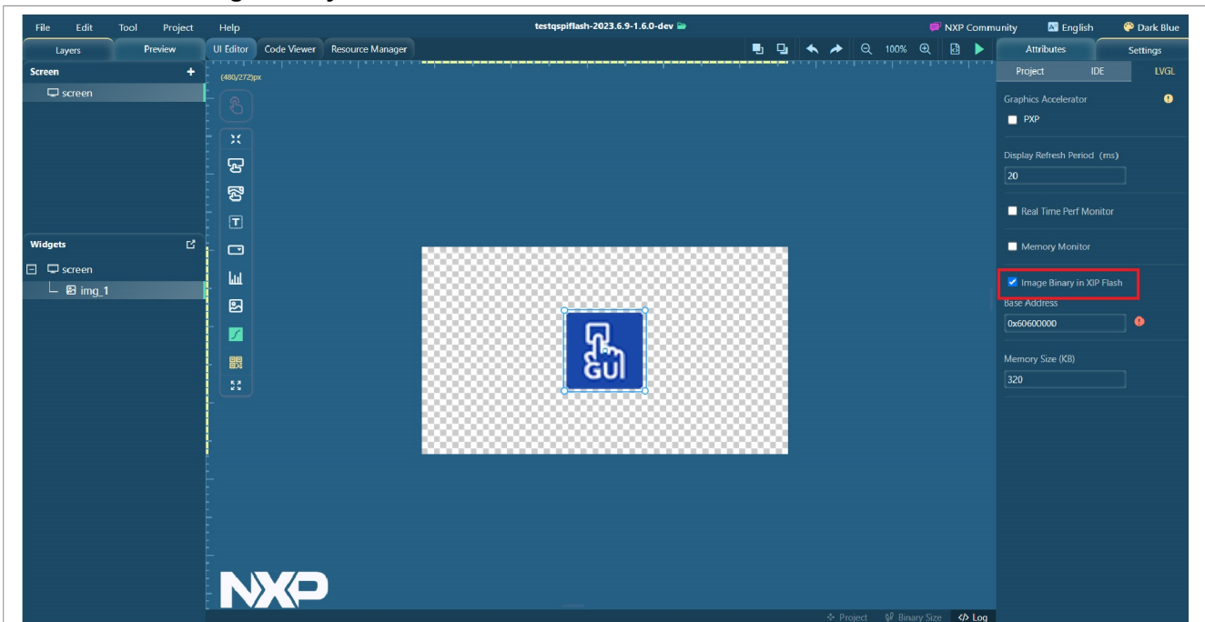
Figure 183. Deselect Image Binary in XIP Flash
