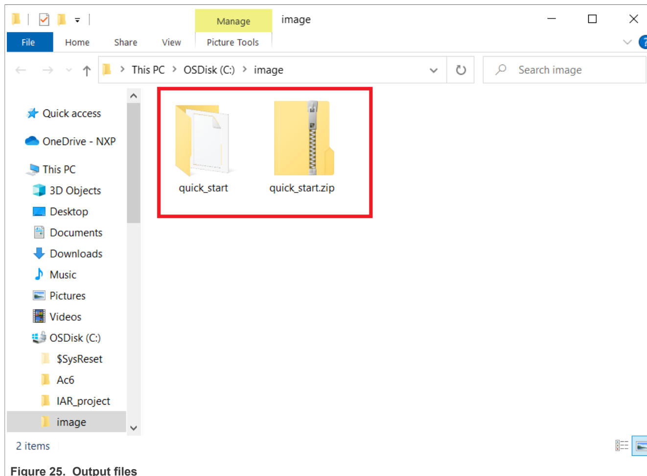
Figure 25. Output files
