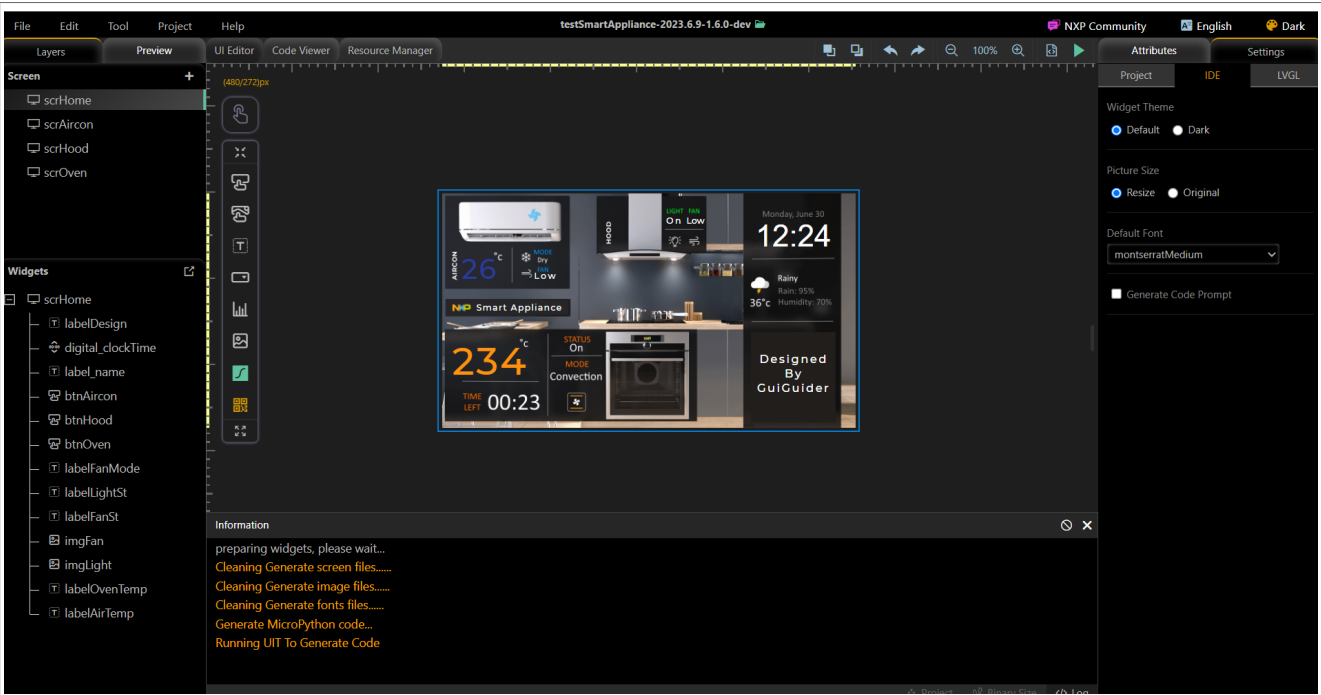
Figure 46. Dark theme
