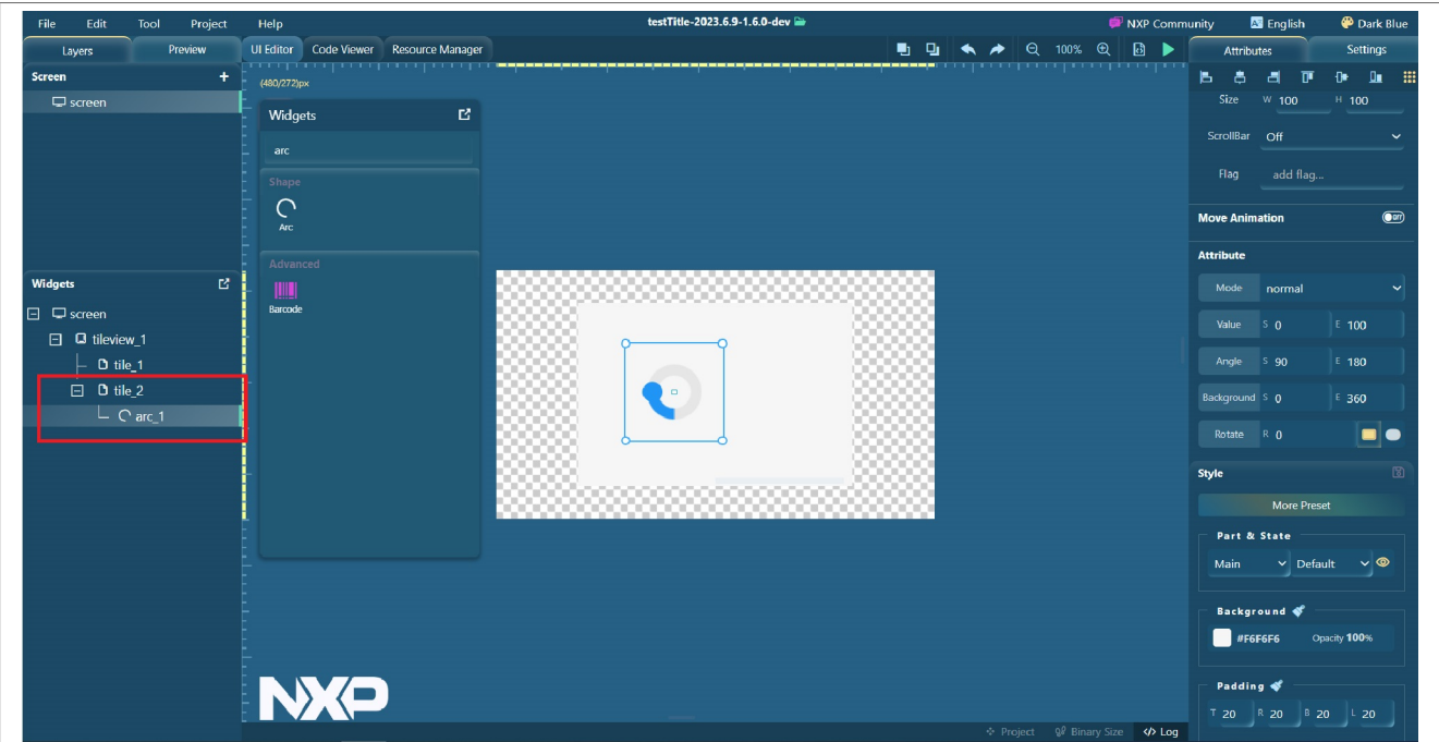
Figure 34. Arc widget
