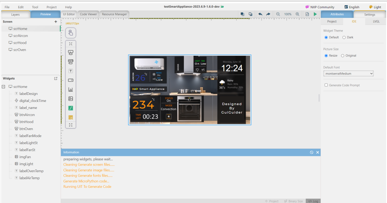
Figure 45. Light theme
