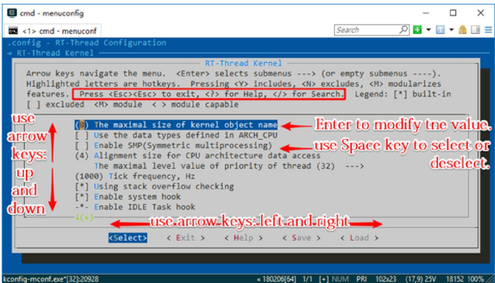
Figure 152. menuconfig
