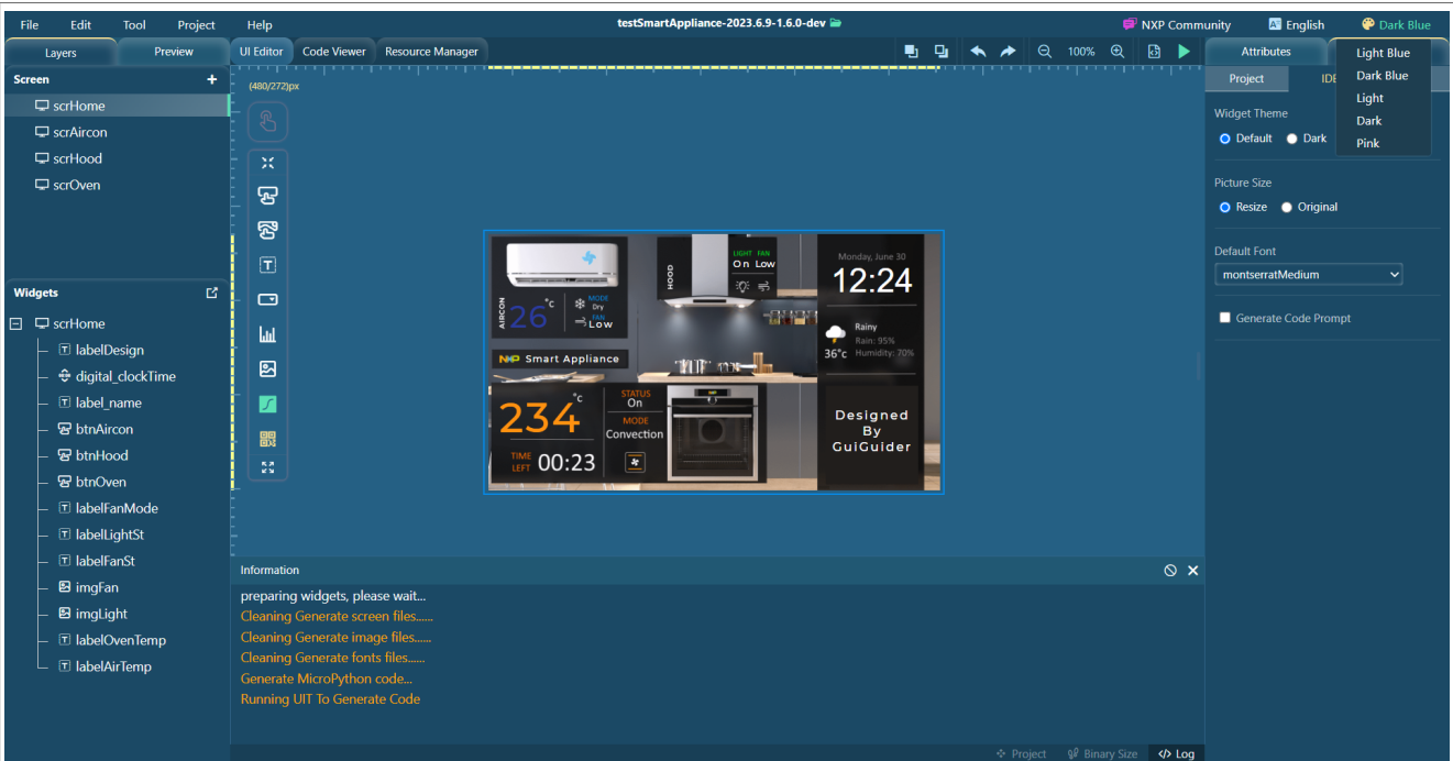
Figure 43. IDE setting
