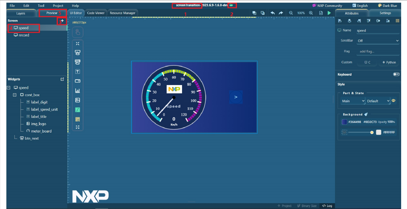
Figure 39. Resource window
