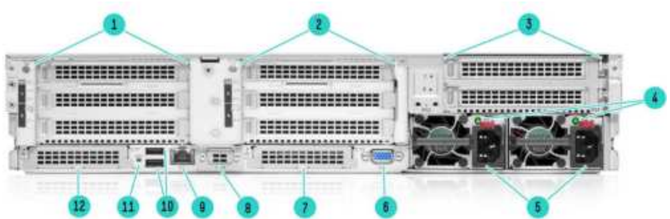
HPE Alletra Storage Server 4120 Configure-to-order System Rear View
