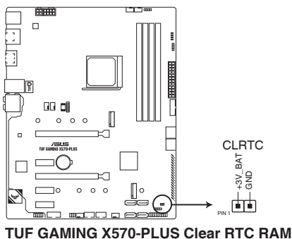
TUF GAMING X570-PLUS Clear RTC RAM
