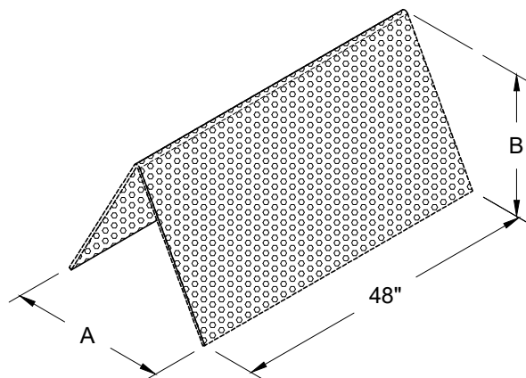
Face View
