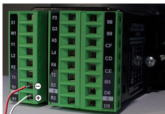
Figure 2: Thermocouple Input Wiring Example
