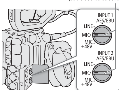
INPUT 1 / INPUT 2 switches (audio source selection)
