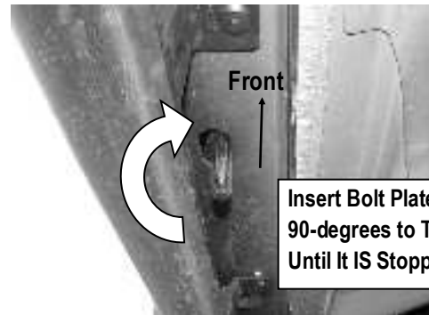
(Fig 3) Insert M10 Bolt Plate into the Slot
