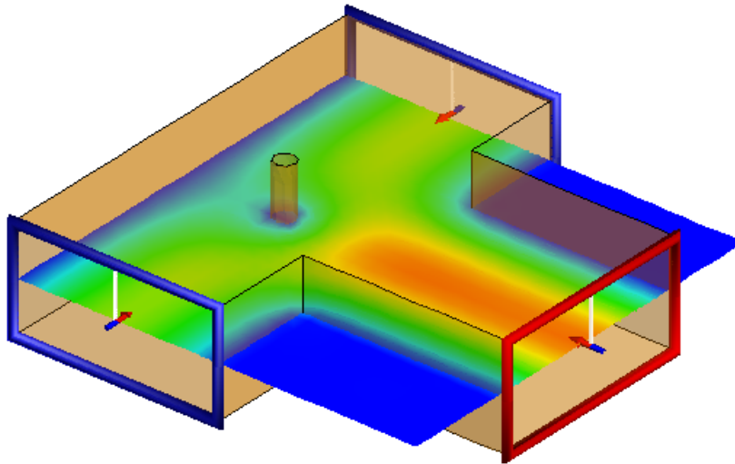
Figure 127: The waveguide power divider and instantaneous near field.
