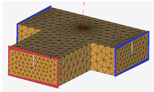
Figure 150: Note the localised mesh refinement at the waveguide port faces.
