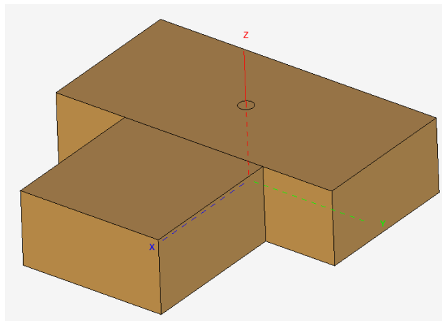
Figure 135: The two waveguide sections and power dividing pin.
