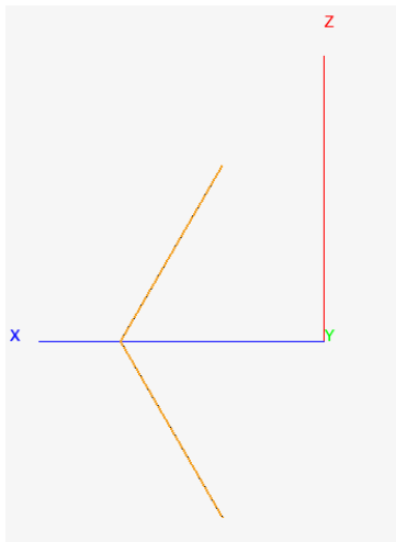
Figure 158: The bent dipole with corner point on the X axis.
