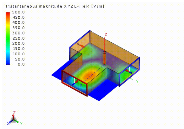
Figure 152: The near field in the power divider (refer to the WebHelp to view the animation of the instantaneous magnitude).
