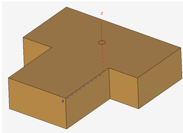
Figure 139: The waveguide section after the redundant faces were removed.
