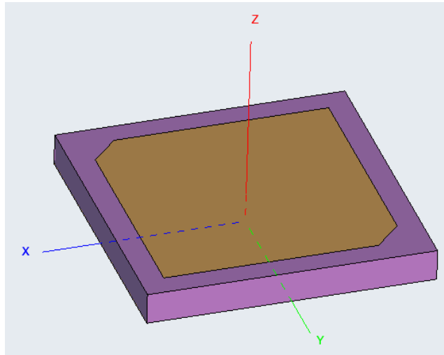
Figure 54: The chamfered GPS patch antenna on a finite substrate.
