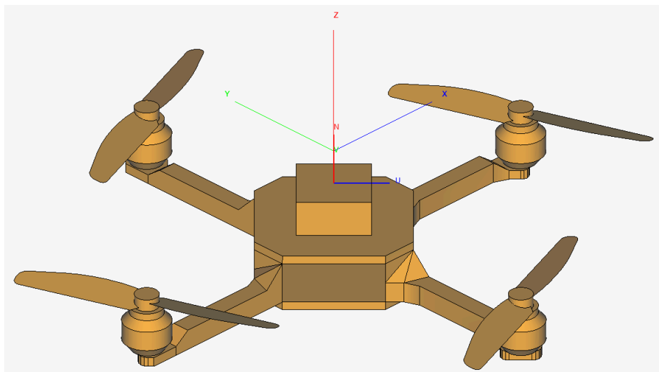
Figure 104: Workplane1 is "aligned" to the top centre of the quadcopter.
