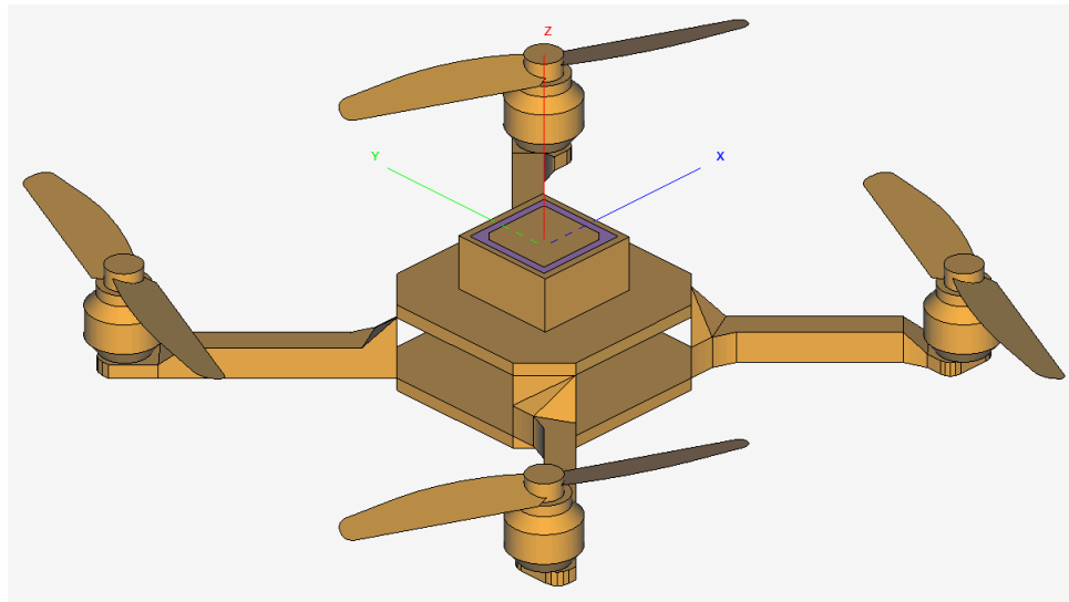
Figure 106: The GPS patch antenna placed on the quadcopter.
