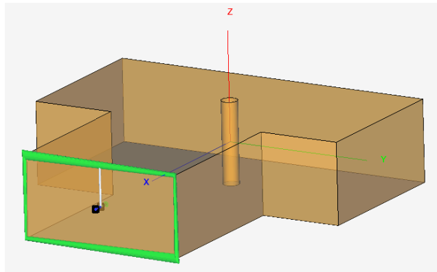
Figure 145: The preview of the waveguide port is displayed in green.
