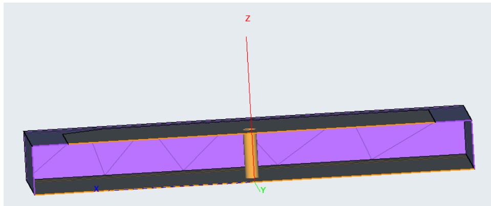
Figure 81: The cutplane shows a cross-sectional view of the patch substrate. Note the thick feedpin as specified by the Wire segment radius .
