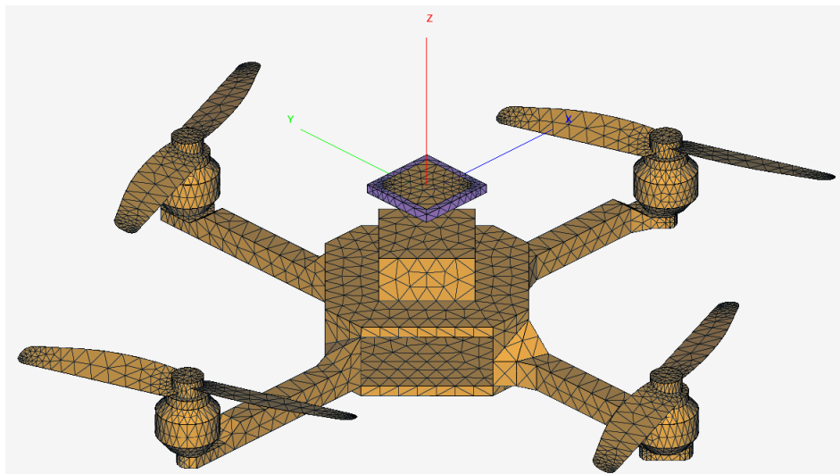
Figure 98: The imported GPS patch model above the quadcopter.
