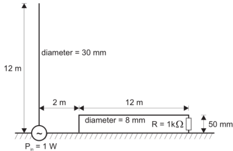
Figure 108: The monopole antenna and the loaded transmission line above an infinite ground plane.
