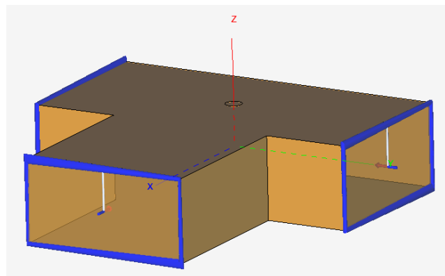
Figure 146: The waveguide power divider with three defined waveguide ports.
