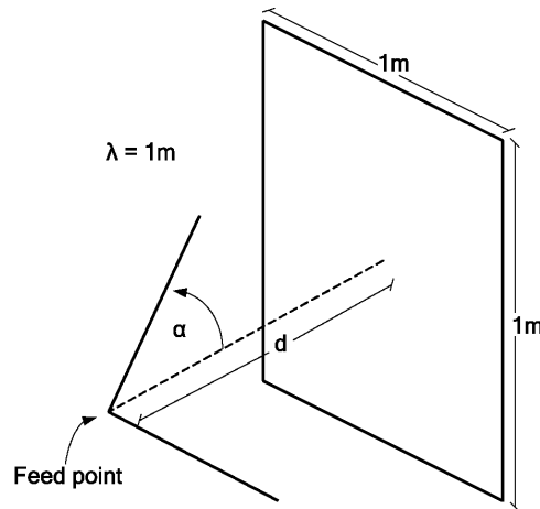
Figure 153: Sketch of the model showing dimensions and other relevant parameters.
