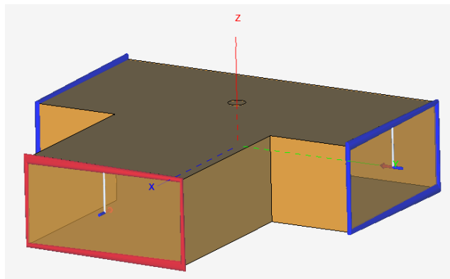
Figure 148: A port with a source is indicated in red.
