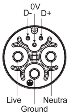
Input - panel connector (front view)
