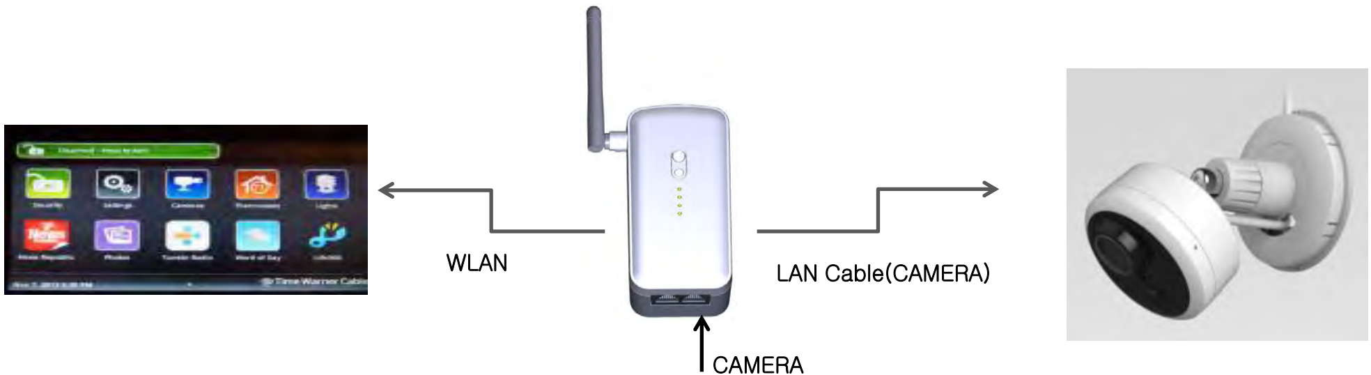
Fig 4. Login connection
