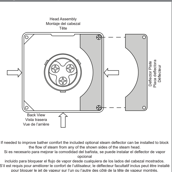
Figure 12 - Optional Deflector
