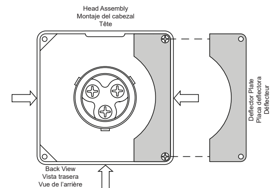
Figure 12 - Optional Deflector
