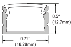
MOFT-CHAN-SLV-6.5 Anodized Aluminum Extrusion, available in 6.5' lengths
