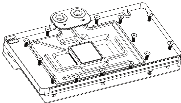
Alphacool Core GeForce RTX 4090 Master with Backplate
