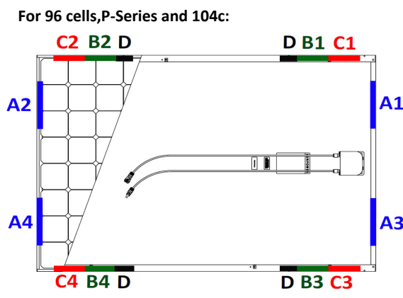
Figure 2: Mounting Zone locations for SunPower modules
