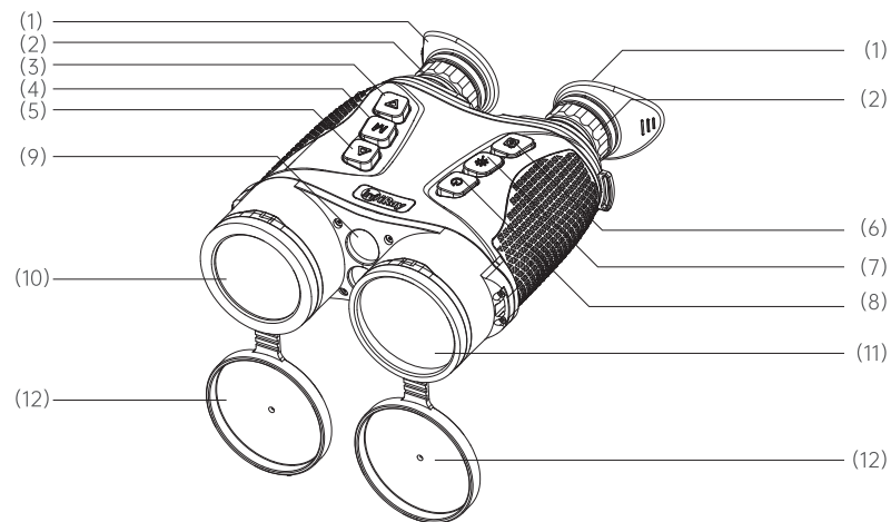
Figure 1 Front View
