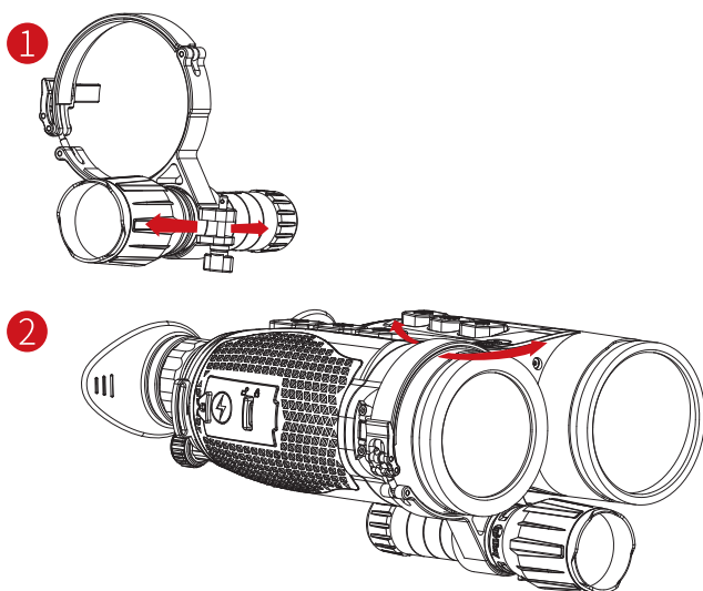
Figure 5 IR Illuminator Mounting Illustrations
