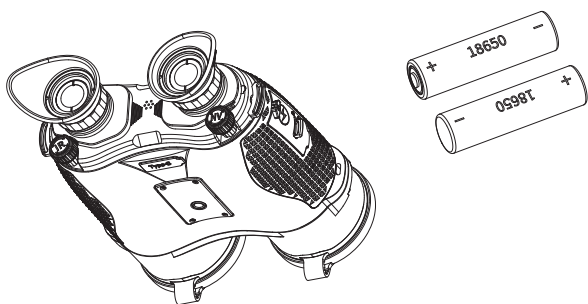
Figure 3 Types of Power Supply
