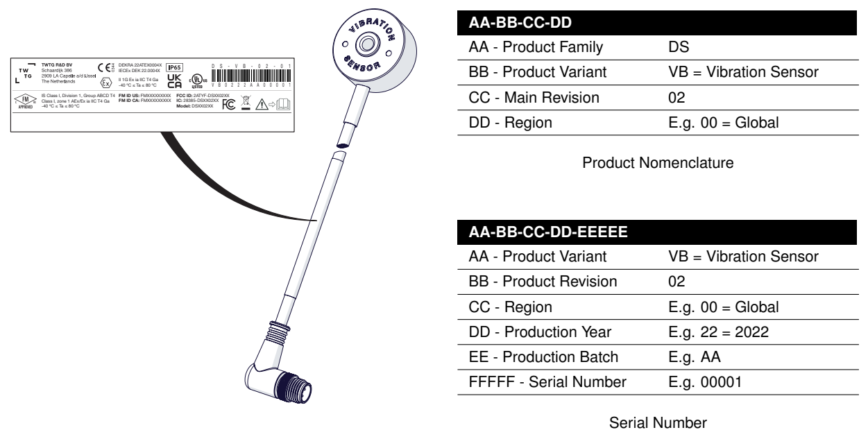
Figure 2: Vibration Sensor product identification
