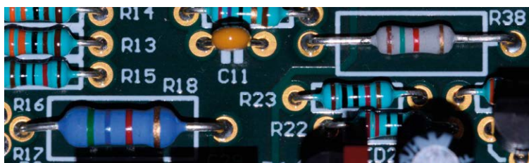
Figure 40. Detail: 1-watt resistors R18 and R38 — notice the size of R38.
