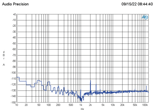
Figure 39. FFT of 1 kHz at 1 W and an 8 \Omega load.
