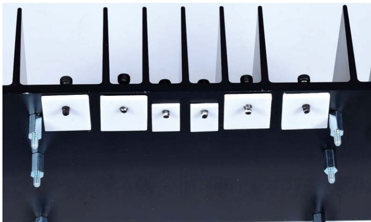
Figure 30. Slide the ceramic washers (pads) over the screw threads before positioning the PCB with the transistors.
