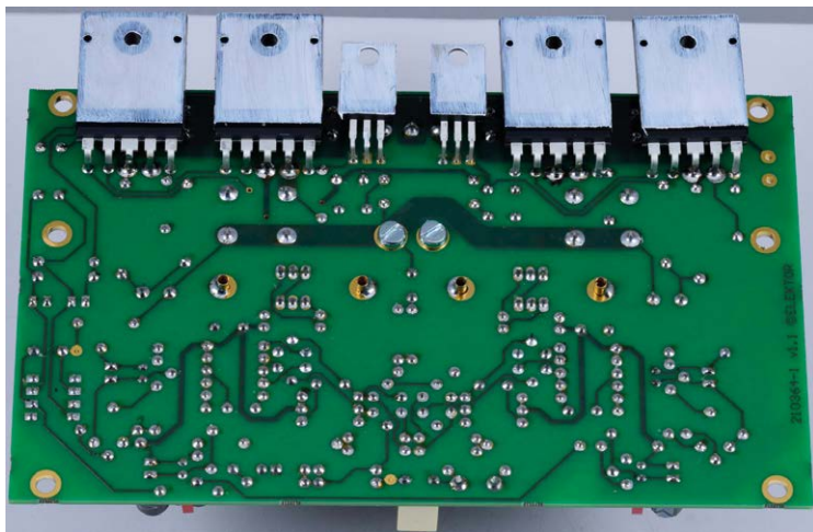
Figure 29. The output stage transistors are soldered, and thermal grease is applied to their backs.
