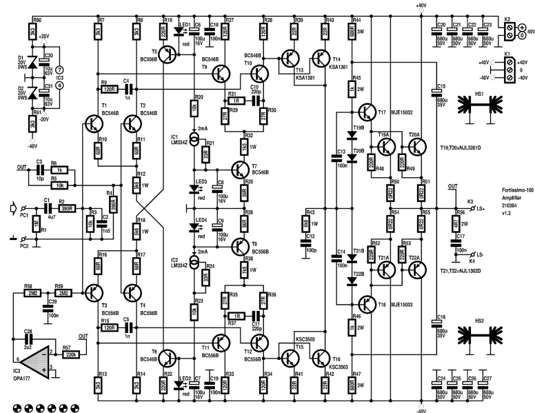
Figure 41. Schematic of the amplifier (210364-1 v1.2).
