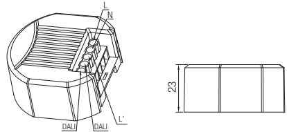
Dimensions(mm)
